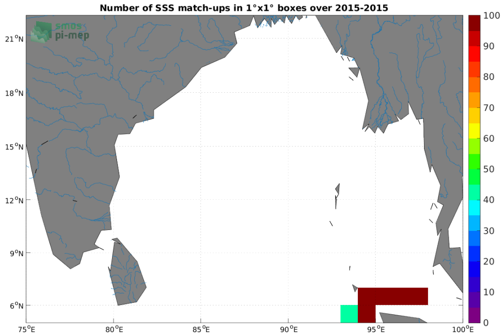
Figure 4: Number of SSS match-ups between TSG (SAMOS) SSS and the SMAP SSS L4 OI v2 - 7 Days (ESR) SSS product for the Ganga and Brahmaputra river plumes Pi-MEP region over 1°×1° boxes and for the full satellite product period.
