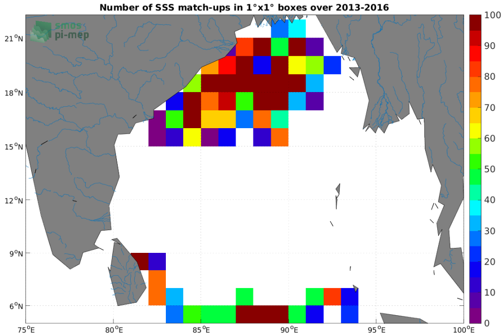
Figure 3: Number of SSS match-ups between Surface drifters SSS and the SMAP SSS L4 OI v2 - 7 Days (ESR) SSS product for the Ganga and Brahmaputra river plumes Pi-MEP region over 1^\circ \times 1^\circ boxes and for the full satellite product period.
