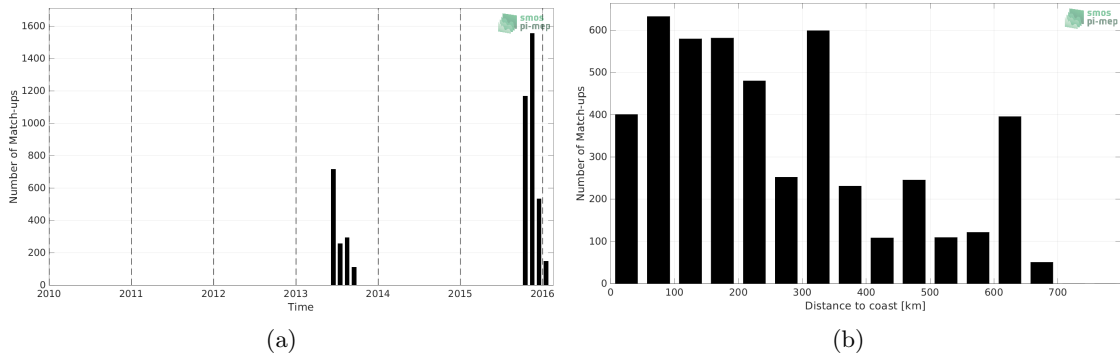
Figure 1: Number of match-ups between Surface drifters and SMAP SSS L4 OI v2 - 7 Days (ESR) SSS as a function of time (a) and as function of the distance to coast (b) over the Ganga and Brahmaputra river plumes Pi-MEP region and for the full satellite product period.
