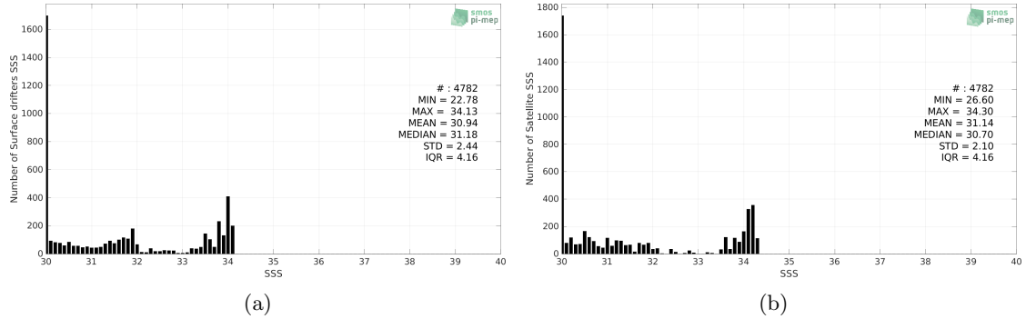
Figure 2: Histograms of SSS from Surface drifters (a) and SMAP SSS L4 OI v2 - 7 Days (ESR) (b) considering all match-up pairs per bins of 0.1 over the Ganga and Brahmaputra river plumes Pi-MEP region and for the full satellite product period.
