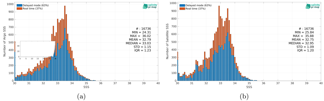
Figure 2: Histograms of SSS from Argo (a) and SMAP SSS L4 OI v2 - 7 Days (ESR) (b) considering all match-up pairs per bins of 0.1 over the Ganga and Brahmaputra river plumes Pi-MEP region and for the full satellite product period.
