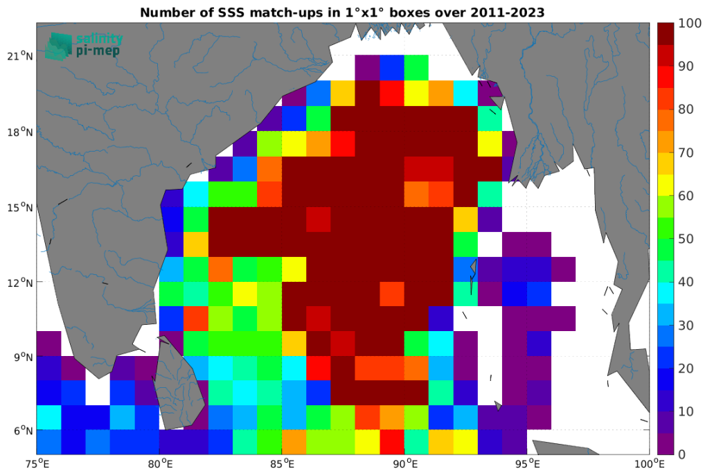
Figure 4: Number of SSS match-ups between Argo SSS and the SMAP SSS L4 OI v2 - 7 Days (ESR) SSS product for the Ganga and Brahmaputra river plumes Pi-MEP region over 1^\circ \times 1^\circ boxes and for the full satellite product period.
