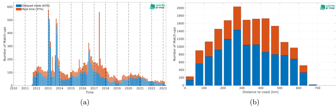
Figure 1: Number of match-ups between Argo and SMAP SSS L4 OI v2 - 7 Days (ESR) SSS as a function of time (a) and as function of the distance to coast (b) over the Ganga and Brahmaputra river plumes Pi-MEP region and for the full satellite product period.
