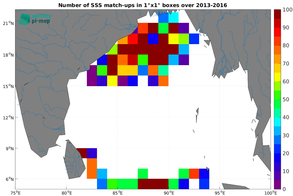
Figure 3: Number of SSS match-ups between Surface drifters SSS and the SMAP SSS L4 OI v2 - Monthly (IPRC) SSS product for the Ganga and Brahmaputra river plumes Pi-MEP region over 1^\circ \times 1^\circ boxes and for the full satellite product period.
