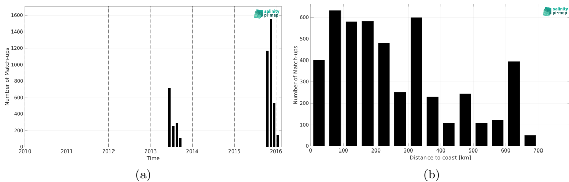
Figure 1: Number of match-ups between Surface drifters and SMAP SSS L4 OI v2 - Monthly (IPRC) SSS as a function of time (a) and as function of the distance to coast (b) over the Ganga and Brahmaputra river plumes Pi-MEP region and for the full satellite product period.
