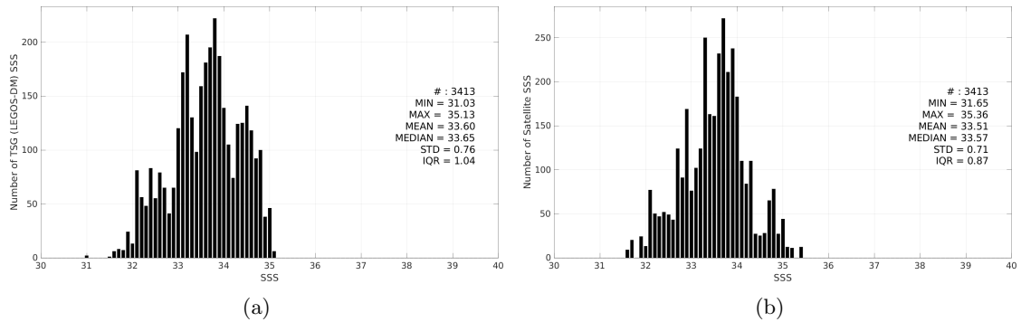
Figure 3: Histograms of SSS from TSG (LEGOS-DM) (a) and SMAP SSS L3 v6 - 8-Day running (RSS) (b) considering all match-up pairs per bins of 0.1 over the Ganga and Brahmaputra river plumes Pi-MEP region and for the full satellite product period.
