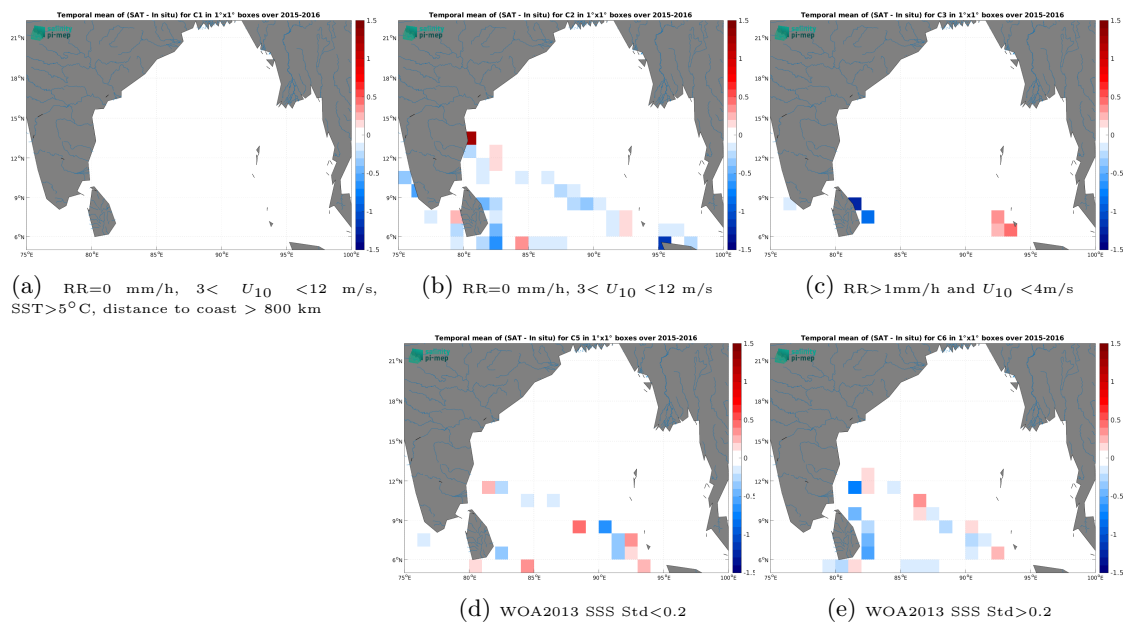
Figure 14: Temporal mean gridded over spatial boxes of size 1^\circ \times 1^\circ of \Delta SSS (SMAP SSS L3 v6 - 8-Day running (RSS) - TSG (LEGOS-DM)) for 5 different subdatasets corresponding to:RR=0 mm/h, 3 < U_{10} < 12 m/s, SST >5^\circ C, distance to coast > 800 km (a), RR=0 mm/h, 3 < U_{10} < 12 m/s (b), RR >1 mm/h and U_{10} < 4 m/s (c), WOA2013 SSS Std <0.2 (d), WOA2013 SSS Std >0.2 (e).
