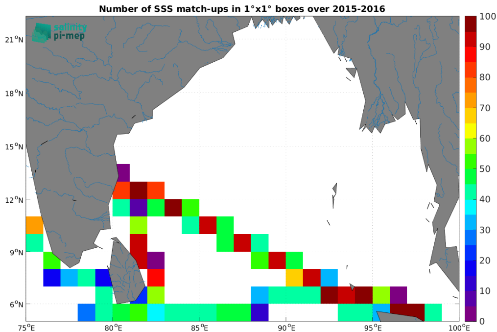
Figure 5: Number of SSS match-ups between TSG (LEGOS-DM) SSS and the SMAP SSS L3 v6 - 8-Day running (RSS) SSS product for the Ganga and Brahmaputra river plumes Pi-MEP region over 1^{\circ} \times 1^{\circ} boxes and for the full satellite product period.
