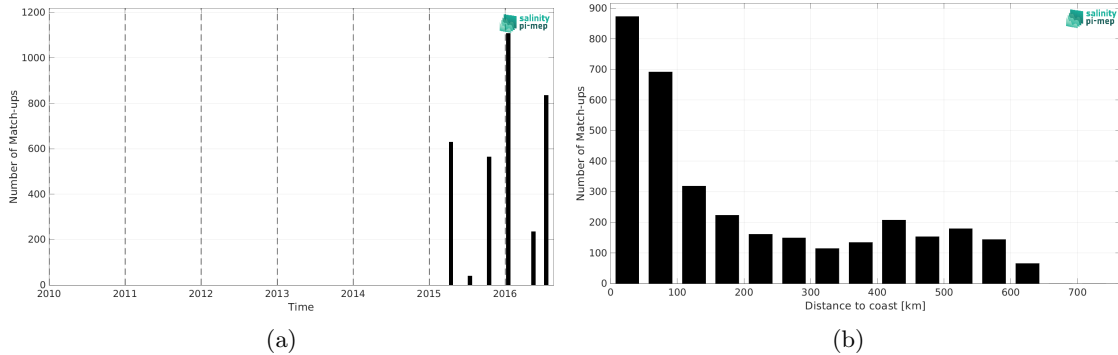
Figure 2: Number of match-ups between TSG (LEGOS-DM) and SMAP SSS L3 v6 - 8-Day running (RSS) SSS as a function of time (a) and as function of the distance to coast (b) over the Ganga and Brahmaputra river plumes Pi-MEP region and for the full satellite product period.
