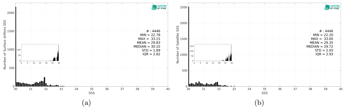
Figure 3: Histograms of SSS from Surface drifters (a) and SMAP SSS L3 v6 - 8-Day running (RSS) (b) considering all match-up pairs per bins of 0.1 over the Ganga and Brahmaputra river plumes Pi-MEP region and for the full satellite product period.
