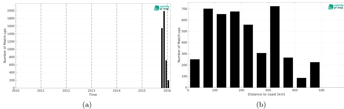
Figure 2: Number of match-ups between Surface drifters and SMAP SSS L3 v6 - 8-Day running (RSS) SSS as a function of time (a) and as function of the distance to coast (b) over the Ganga and Brahmaputra river plumes Pi-MEP region and for the full satellite product period.
