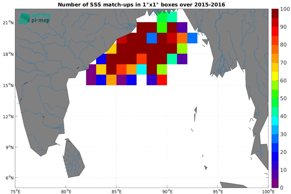
Figure 4: Number of SSS match-ups between Surface drifters SSS and the SMAP SSS L3 v6 - Monthly (RSS) SSS product for the Ganga and Brahmaputra river plumes Pi-MEP region over 1^\circ \times 1^\circ boxes and for the full satellite product period.
