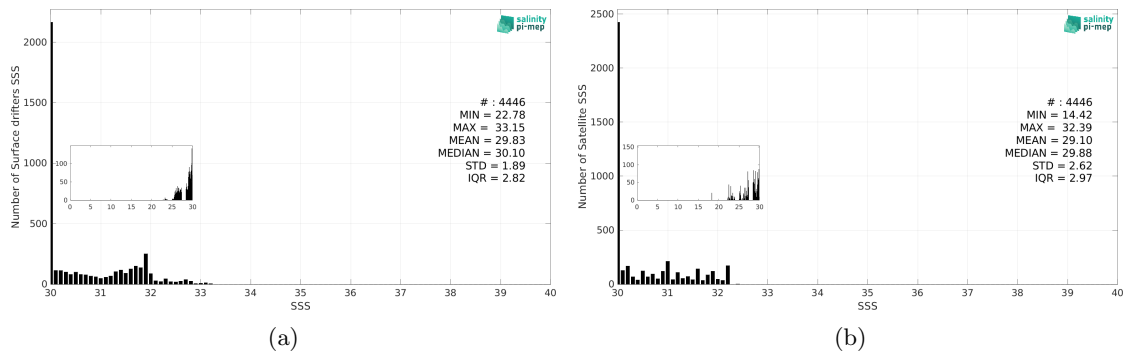
Figure 3: Histograms of SSS from Surface drifters (a) and SMAP SSS L3 v6 - Monthly (RSS) (b) considering all match-up pairs per bins of 0.1 over the Ganga and Brahmaputra river plumes Pi-MEP region and for the full satellite product period.
