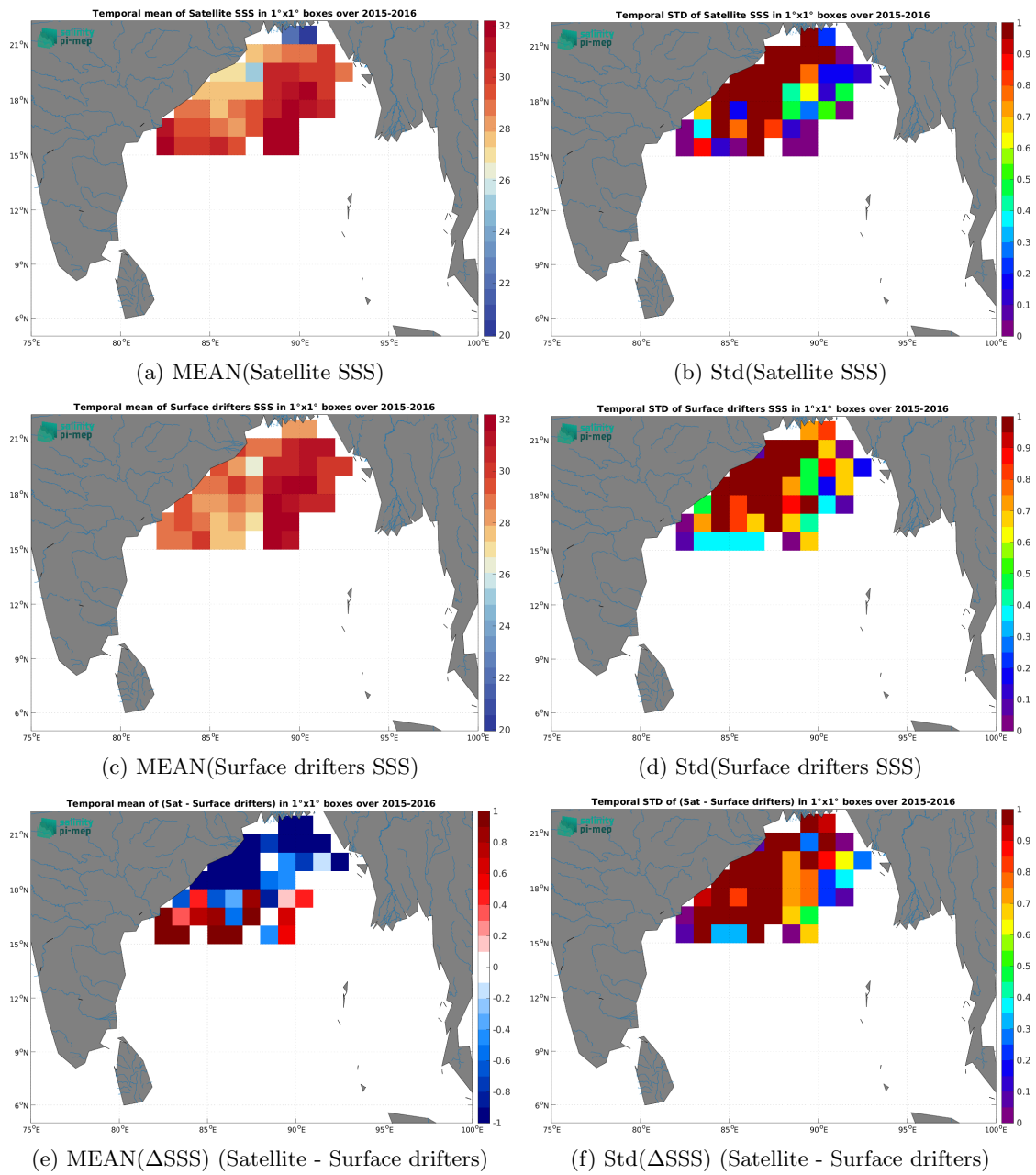
Figure 6: Temporal mean (left) and Std (right) of SSS from SMAP SSS L3 v6 - Monthly (RSS) (top), Surface drifters (middle), and of \Delta SSS (Satellite - Surface drifters). Only match-up pairs are used to generate these maps.
