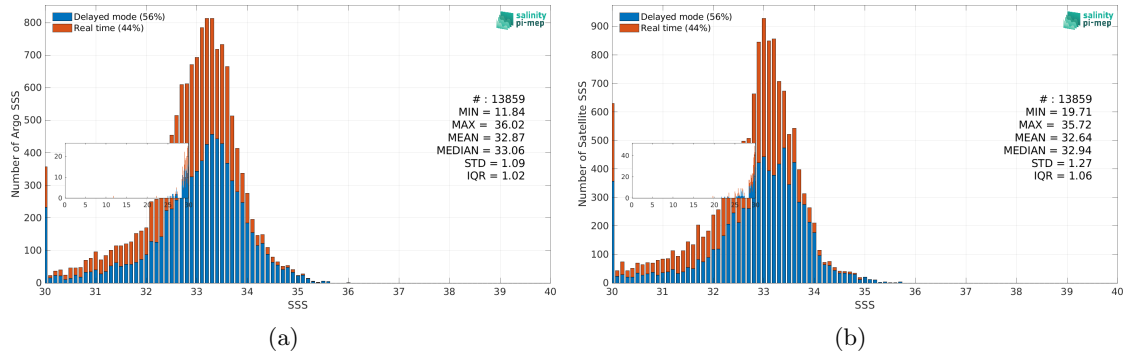
Figure 3: Histograms of SSS from Argo (a) and SMAP SSS L3 v6 - Monthly (RSS) (b) considering all match-up pairs per bins of 0.1 over the Ganga and Brahmaputra river plumes Pi-MEP region and for the full satellite product period.
