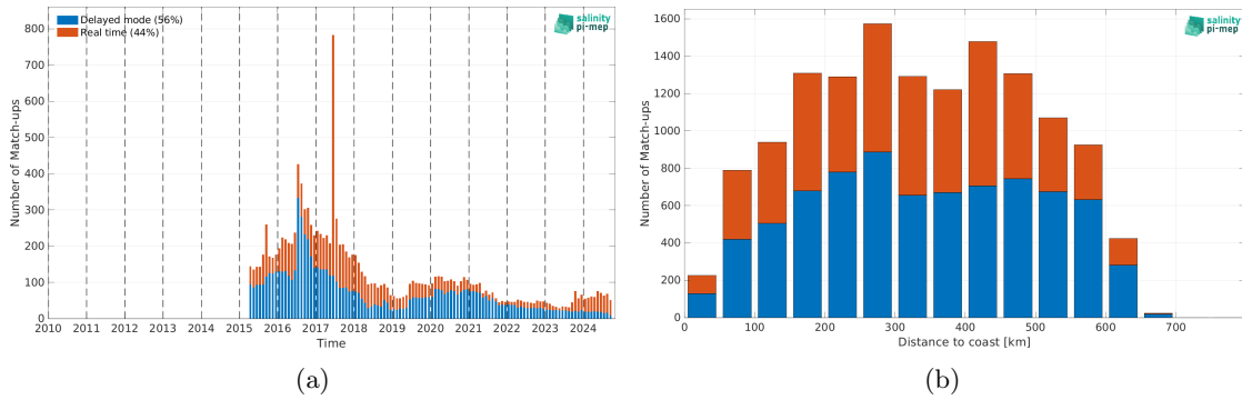
Figure 2: Number of match-ups between Argo and SMAP SSS L3 v6 - Monthly (RSS) SSS as a function of time (a) and as function of the distance to coast (b) over the Ganga and Brahmaputra river plumes Pi-MEP region and for the full satellite product period.
