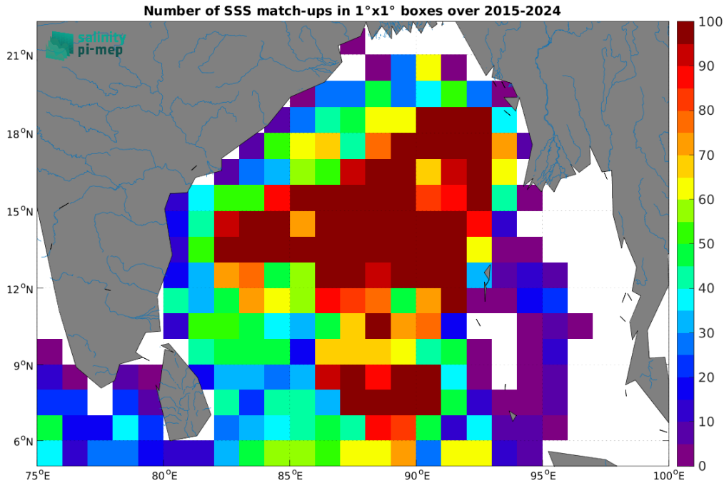
Figure 5: Number of SSS match-ups between Argo SSS and the SMAP SSS L3 v6 - Monthly (RSS) SSS product for the Ganga and Brahmaputra river plumes Pi-MEP region over 1^\circ \times 1^\circ boxes and for the full satellite product period.
