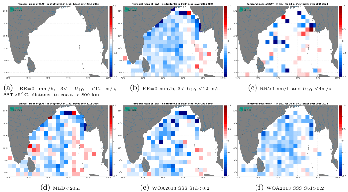
Figure 14: Temporal mean gridded over spatial boxes of size 1^\circ \times 1^\circ of \Delta SSS (SMAP SSS L3 v6 - Monthly (RSS) - Argo) for 6 different subdatasets corresponding to:RR=0 mm/h, 3 < U_{10} < 12 m/s, SST>5°C, distance to coast > 800 km (a), RR=0 mm/h, 3 < U_{10} < 12 m/s (b), RR>1mm/h and U_{10} < 4 m/s (c),MLD<20m (d),WOA2013 SSS Std<0.2 (e),WOA2013 SSS Std>0.2 (f).
