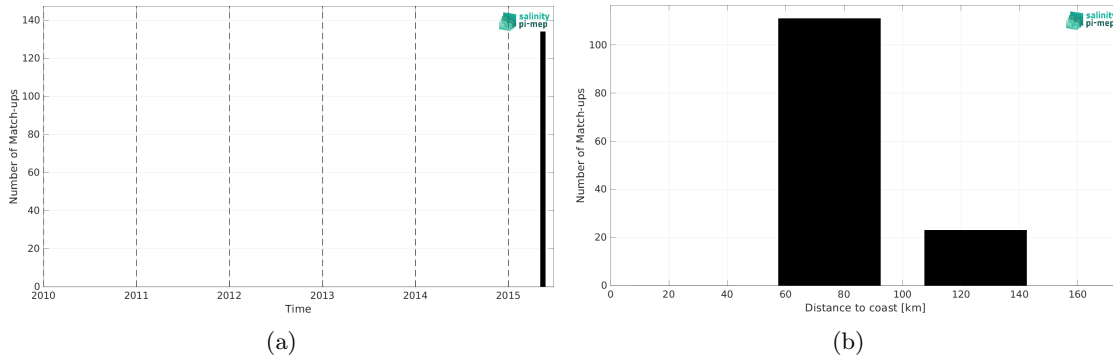
Figure 2: Number of match-ups between TSG (SAMOS) and SMAP SSS L3 v5.3 - Monthly (RSS) SSS as a function of time (a) and as function of the distance to coast (b) over the Ganga and Brahmaputra river plumes Pi-MEP region and for the full satellite product period.
