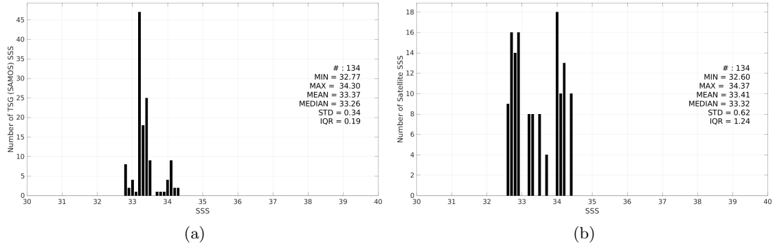
Figure 3: Histograms of SSS from TSG (SAMOS) (a) and SMAP SSS L3 v5.3 - Monthly (RSS) (b) considering all match-up pairs per bins of 0.1 over the Ganga and Brahmaputra river plumes Pi-MEP region and for the full satellite product period.
