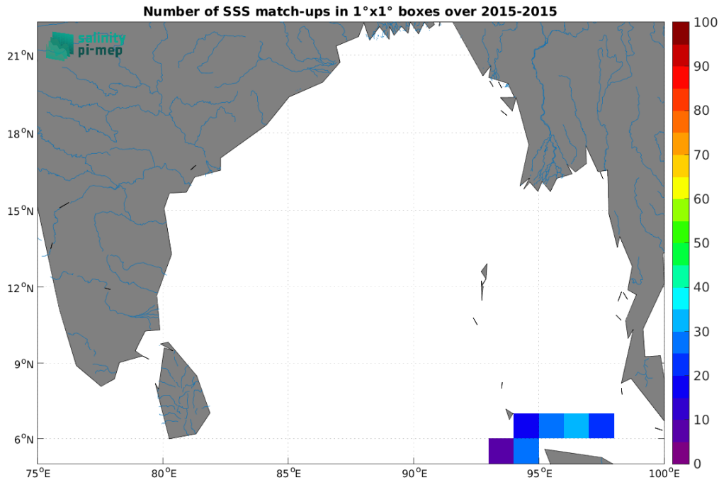
Figure 5: Number of SSS match-ups between TSG (SAMOS) SSS and the SMAP SSS L3 v5.3 - Monthly (RSS) SSS product for the Ganga and Brahmaputra river plumes Pi-MEP region over 1^{\circ} \times 1^{\circ} boxes and for the full satellite product period.
