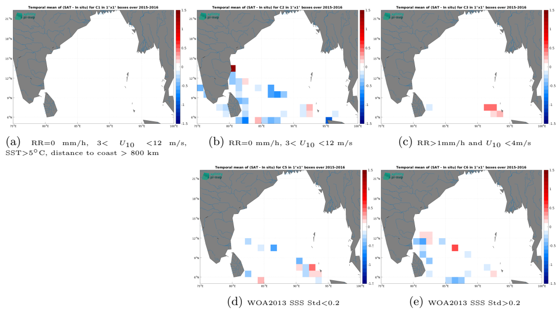
Figure 14: Temporal mean gridded over spatial boxes of size 1^\circ \times 1^\circ of \Delta SSS (SMAP SSS L3 v5.3 - Monthly (RSS) - TSG (LEGOS-DM)) for 5 different subdatasets corresponding to:RR=0 mm/h, 3 < U_{10} < 12 m/s, SST >5^\circ C, distance to coast > 800 km (a), RR=0 mm/h, 3 < U_{10} < 12 m/s (b), RR >1 mm/h and U_{10} < 4 m/s (c), WOA2013 SSS Std <0.2 (d), WOA2013 SSS Std >0.2 (e).
