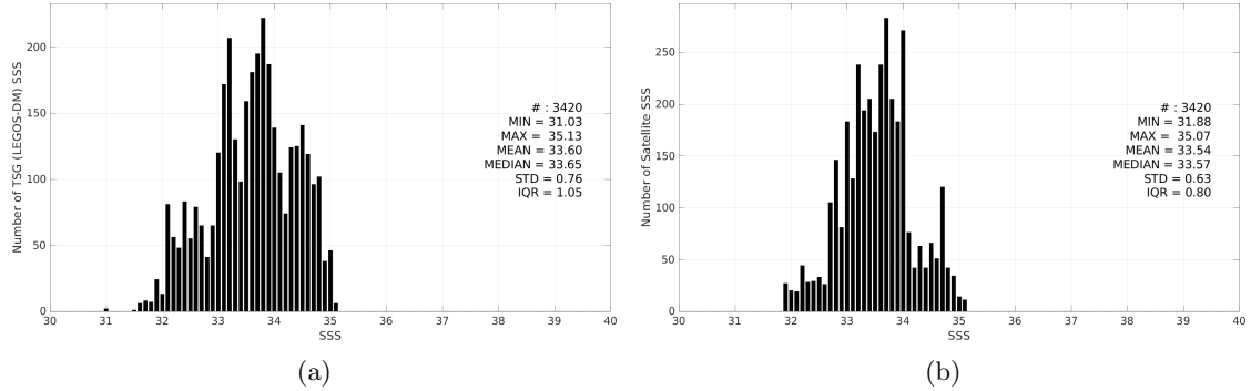
Figure 3: Histograms of SSS from TSG (LEGOS-DM) (a) and SMAP SSS L3 v5.3 - Monthly (RSS) (b) considering all match-up pairs per bins of 0.1 over the Ganga and Brahmaputra river plumes Pi-MEP region and for the full satellite product period.
