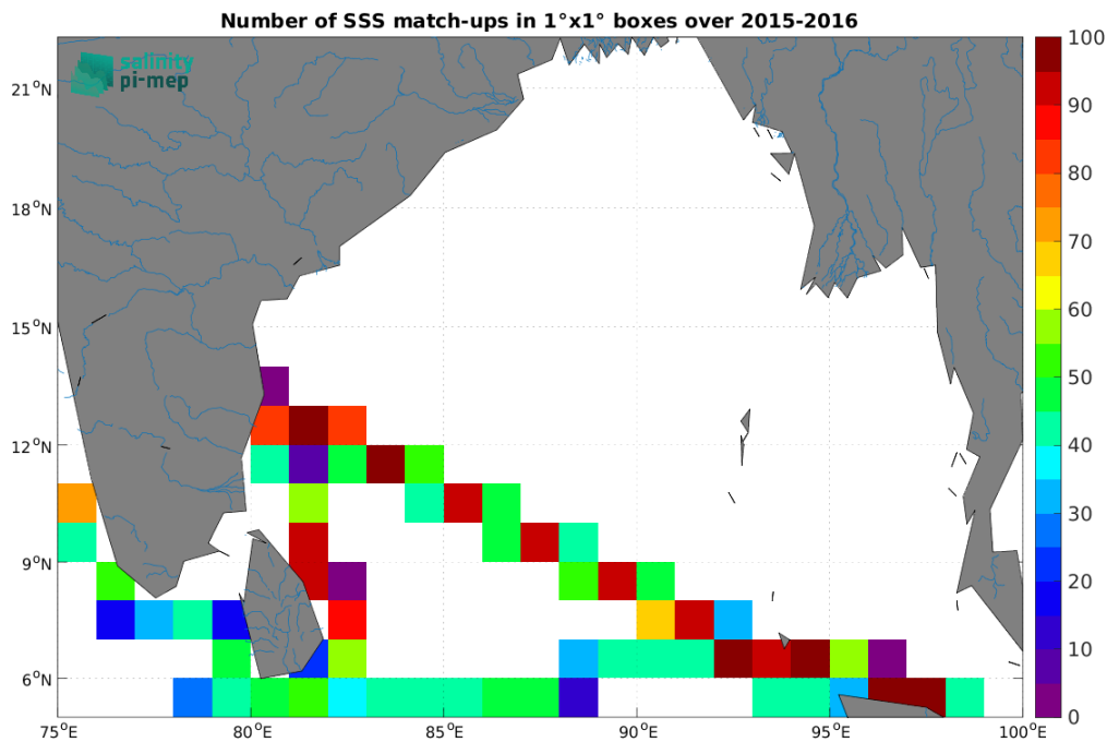
Figure 5: Number of SSS match-ups between TSG (LEGOS-DM) SSS and the SMAP SSS L3 v5.3 - Monthly (RSS) SSS product for the Ganga and Brahmaputra river plumes Pi-MEP region over 1^\circ \times 1^\circ boxes and for the full satellite product period.
