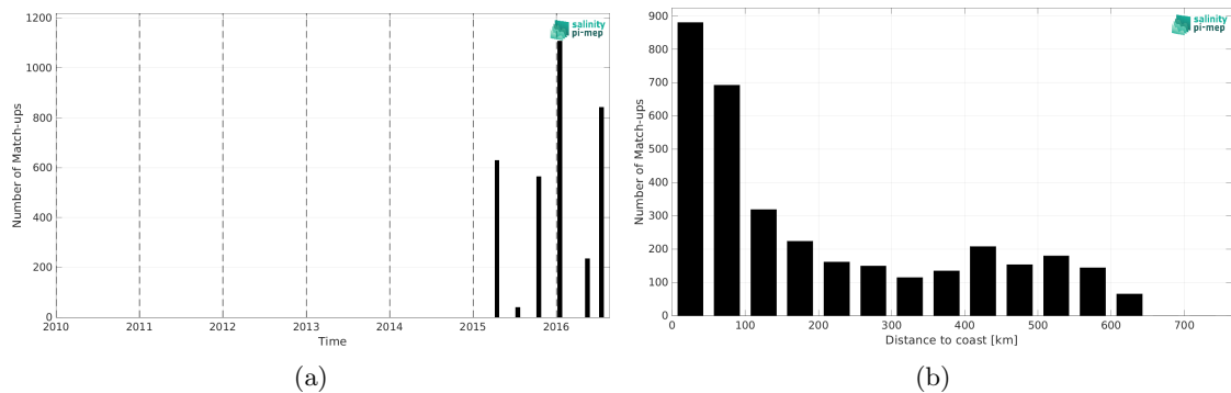
Figure 2: Number of match-ups between TSG (LEGOS-DM) and SMAP SSS L3 v5.3 - Monthly (RSS) SSS as a function of time (a) and as function of the distance to coast (b) over the Ganga and Brahmaputra river plumes Pi-MEP region and for the full satellite product period.
