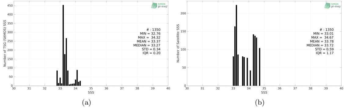
Figure 2: Histograms of SSS from TSG (SAMOS) (a) and SMAP SSS L3 v5 - Monthly (RSS) (b) considering all match-up pairs per bins of 0.1 over the Ganga and Brahmaputra river plumes Pi-MEP region and for the full satellite product period.
