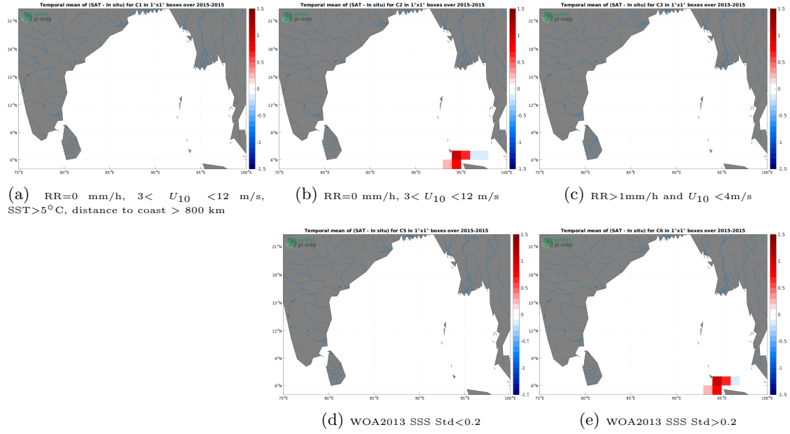
Figure 12: Temporal mean gridded over spatial boxes of size 1^\circ \times 1^\circ of \Delta SSS (SMAP SSS L3 v5 - Monthly (RSS) - TSG (SAMOS)) for 5 different subdatasets corresponding to: RR=0 mm/h, 3 < U_{10} < 12 m/s, SST > 5^\circ C , distance to coast > 800 km (a), RR=0 mm/h, 3 < U_{10} < 12 m/s (b), RR > 1 mm/h and U_{10} < 4 m/s (c), WOA2013 SSS Std < 0.2 (d), WOA2013 SSS Std > 0.2 (e).
