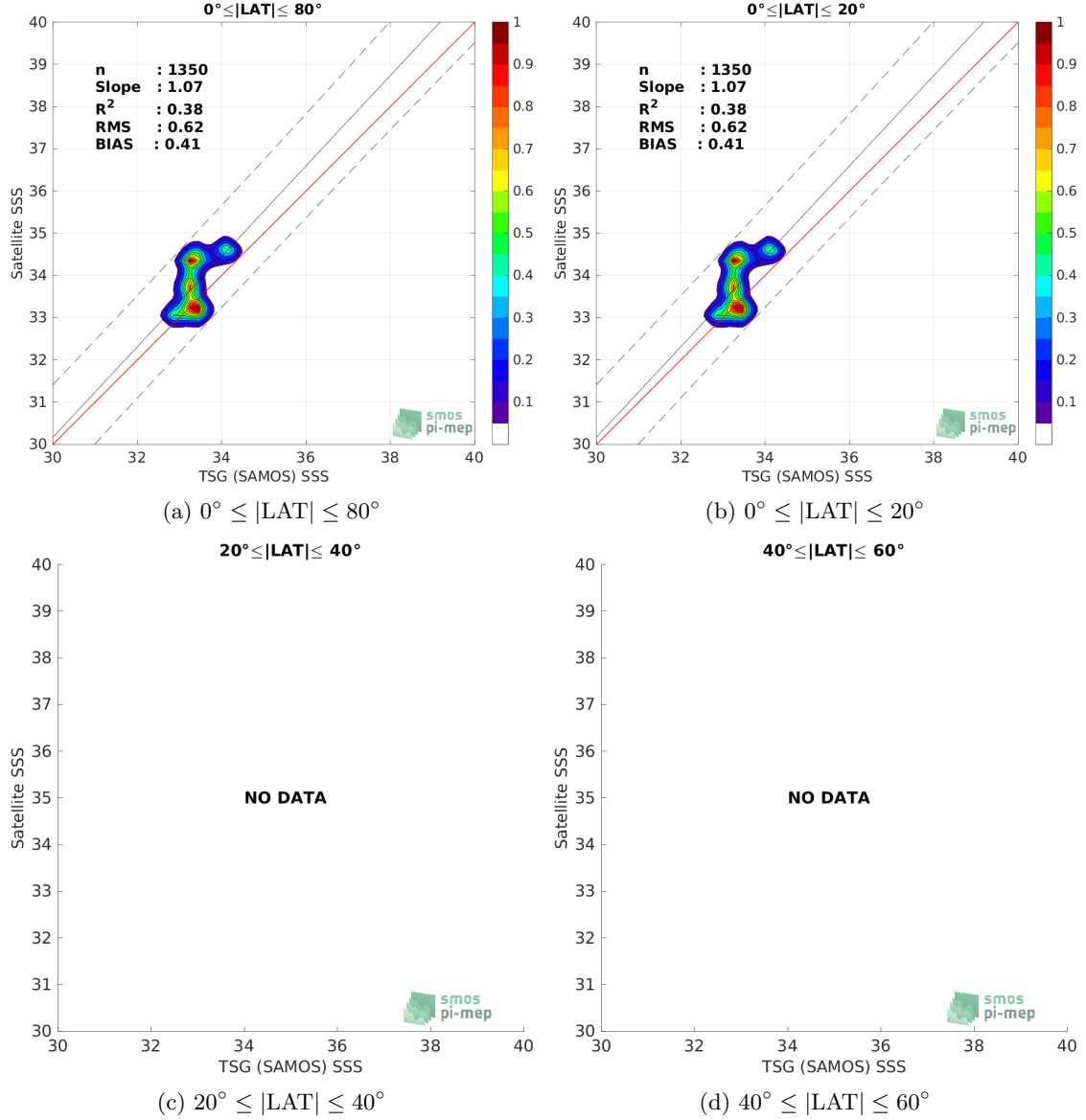
Figure 9: Contour maps of the concentration of SMAP SSS L3 v5 - Monthly (RSS) SSS (y-axis) versus TSG (SAMOS) SSS (x-axis) at match-up pairs for different latitude bands. For each plot, the red line shows x=y . The black thin and dashed lines indicate a linear fit through the data cloud and the \pm 95\% confidence levels, respectively. The number match-up pairs n , the slope and R^2 coefficient of the linear fit, the root mean square (RMS) and the mean bias between satellite and in situ data are indicated for each latitude band in each plots.
