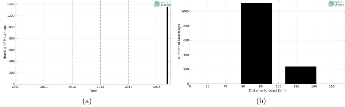
Figure 1: Number of match-ups between TSG (SAMOS) and SMAP SSS L3 v5 - Monthly (RSS) SSS as a function of time (a) and as function of the distance to coast (b) over the Ganga and Brahmaputra river plumes Pi-MEP region and for the full satellite product period.
