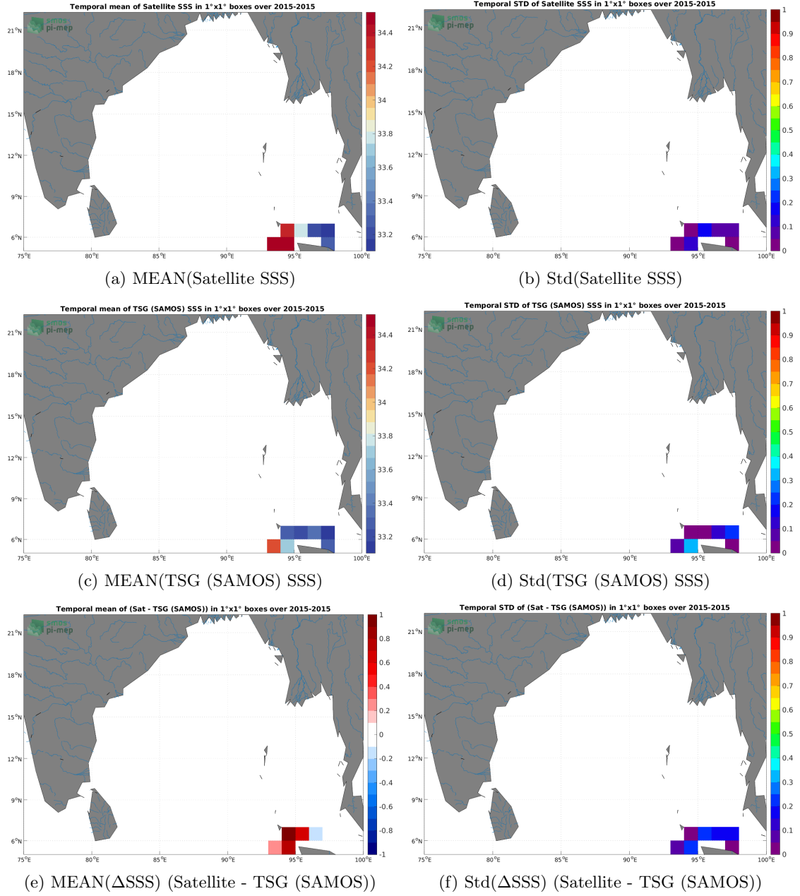
Figure 6: Temporal mean (left) and Std (right) of SSS from SMAP SSS L3 v5 - Monthly (RSS) (top), TSG (SAMOS) (middle), and of \Delta SSS (Satellite - TSG (SAMOS)). Only match-up pairs are used to generate these maps.
