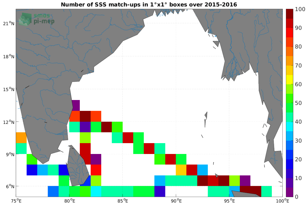
Figure 4: Number of SSS match-ups between TSG (LEGOS-DM) SSS and the SMAP SSS L3 v5 - Monthly (RSS) SSS product for the Ganga and Brahmaputra river plumes Pi-MEP region over 1^\circ \times 1^\circ boxes and for the full satellite product period.
