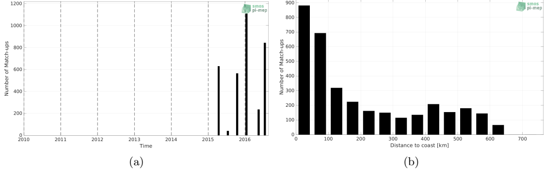
Figure 1: Number of match-ups between TSG (LEGOS-DM) and SMAP SSS L3 v5 - Monthly (RSS) SSS as a function of time (a) and as function of the distance to coast (b) over the Ganga and Brahmaputra river plumes Pi-MEP region and for the full satellite product period.
