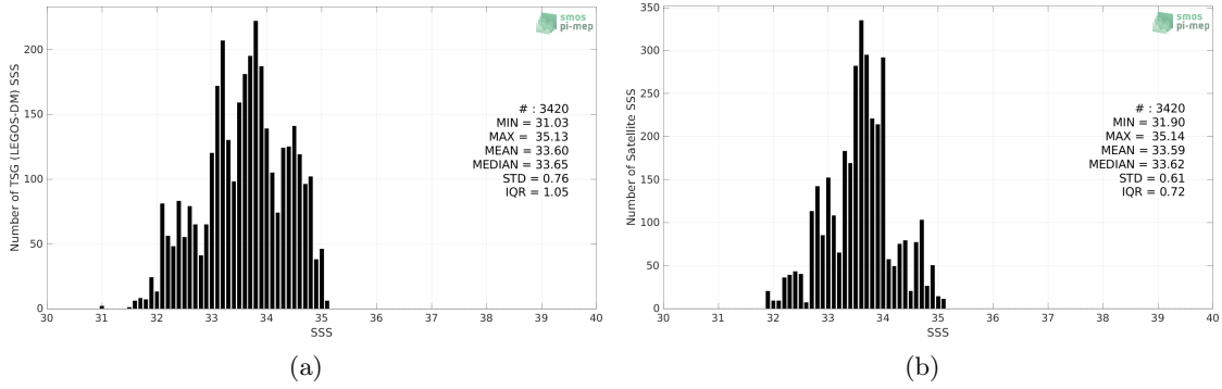
Figure 2: Histograms of SSS from TSG (LEGOS-DM) (a) and SMAP SSS L3 v5 - Monthly (RSS) (b) considering all match-up pairs per bins of 0.1 over the Ganga and Brahmaputra river plumes Pi-MEP region and for the full satellite product period.
