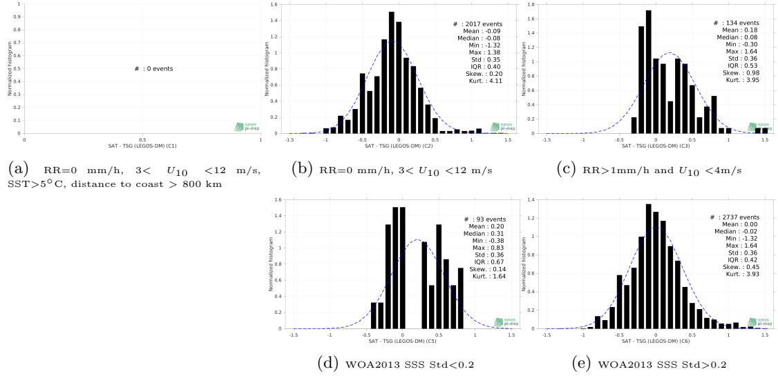
Figure 13: Normalized histogram of \Delta SSS (SMAP SSS L3 v5 - Monthly (RSS) - TSG (LEGOS-DM)) for 5 different subdatasets corresponding to: RR=0 mm/h, 3 < U_{10} < 12 m/s, SST > 5^\circ C , distance to coast > 800 km (a), RR=0 mm/h, 3 < U_{10} < 12 m/s (b), RR > 1 mm/h and U_{10} < 4 m/s (c), WOA2013 SSS Std < 0.2 (d), WOA2013 SSS Std > 0.2 (e).
