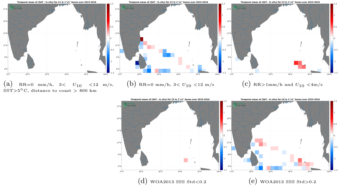
Figure 12: Temporal mean gridded over spatial boxes of size 1^\circ \times 1^\circ of \Delta SSS (SMAP SSS L3 v5 - Monthly (RSS) - TSG (LEGOS-DM)) for 5 different subdatasets corresponding to: RR=0 mm/h, 3 < U_{10} < 12 m/s, SST > 5^\circ C , distance to coast > 800 km (a), RR=0 mm/h, 3 < U_{10} < 12 m/s (b), RR > 1 mm/h and U_{10} < 4 m/s (c), WOA2013 SSS Std < 0.2 (d), WOA2013 SSS Std > 0.2 (e).
