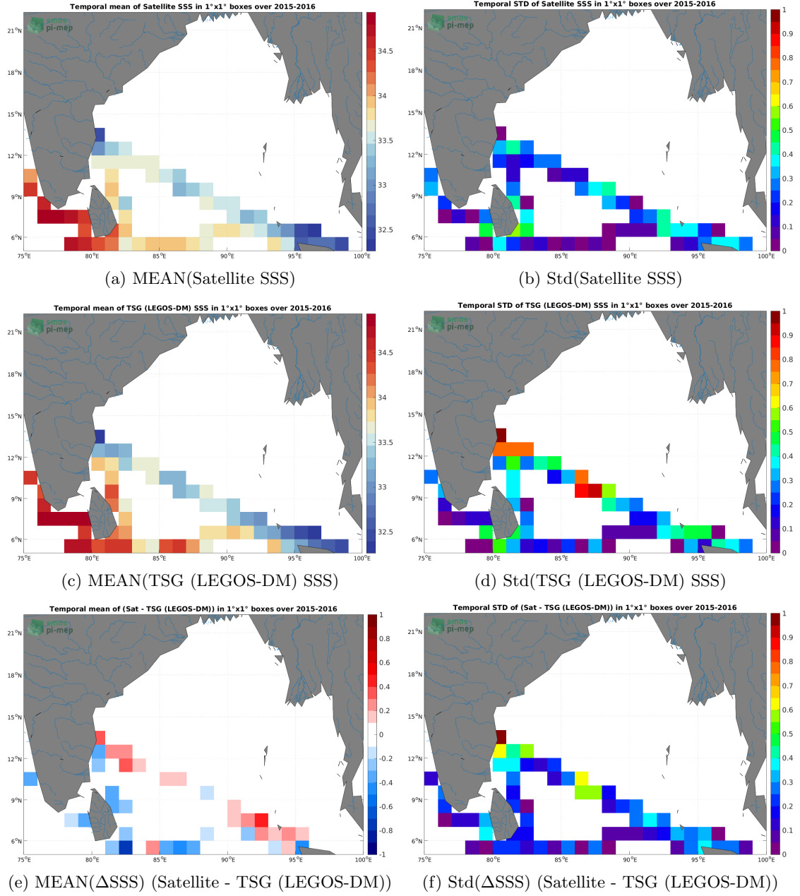
Figure 6: Temporal mean (left) and Std (right) of SSS from SMAP SSS L3 v5 - Monthly (RSS) (top), TSG (LEGOS-DM) (middle), and of \Delta SSS (Satellite - TSG (LEGOS-DM)). Only match-up pairs are used to generate these maps.
