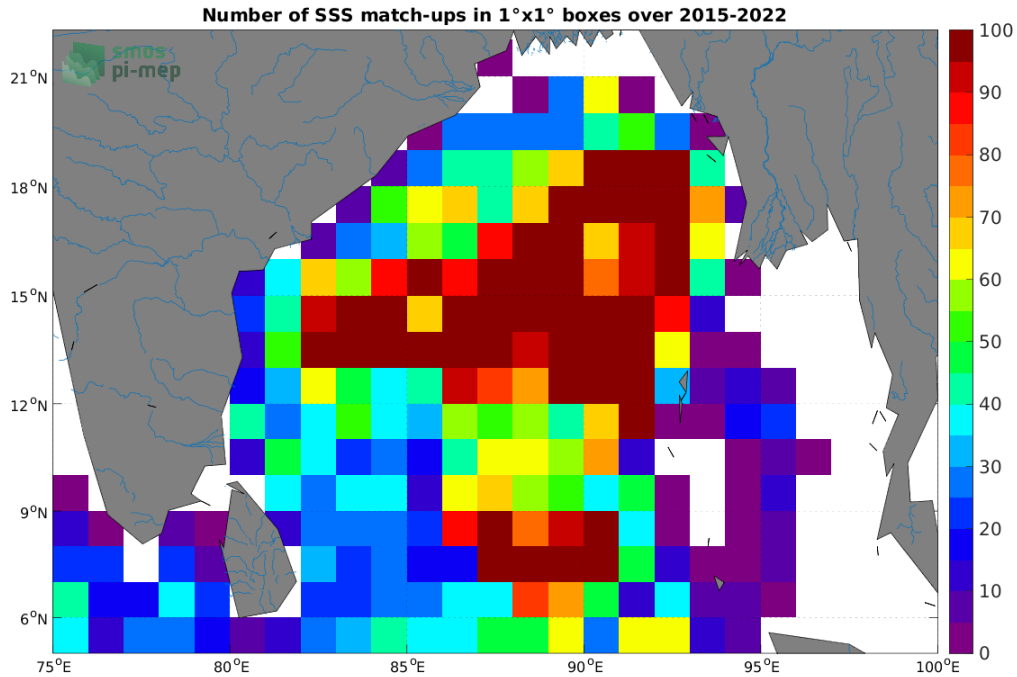
Figure 4: Number of SSS match-ups between Argo SSS and the SMAP SSS L3 v5 - Monthly (RSS) SSS product for the Ganga and Brahmaputra river plumes Pi-MEP region over 1^\circ \times 1^\circ boxes and for the full satellite product period.
