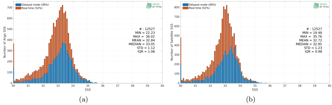
Figure 2: Histograms of SSS from Argo (a) and SMAP SSS L3 v5 - Monthly (RSS) (b) considering all match-up pairs per bins of 0.1 over the Ganga and Brahmaputra river plumes Pi-MEP region and for the full satellite product period.
