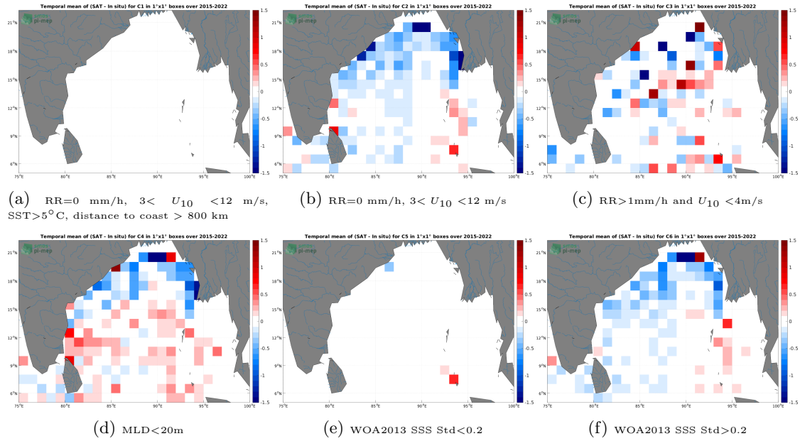
Figure 12: Temporal mean gridded over spatial boxes of size 1^\circ \times 1^\circ of \Delta SSS (SMAP SSS L3 v5 - Monthly (RSS) - Argo) for 6 different subdatasets corresponding to: RR=0 mm/h, 3 < U_{10} < 12 m/s, SST > 5^\circ C , distance to coast > 800 km (a), RR=0 mm/h, 3 < U_{10} < 12 m/s (b), RR > 1 mm/h and U_{10} < 4 m/s (c), MLD < 20 m (d), WOA2013 SSS Std < 0.2 (e), WOA2013 SSS Std > 0.2 (f).
