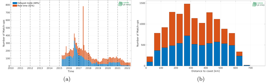
Figure 1: Number of match-ups between Argo and SMAP SSS L3 v5 - Monthly (RSS) SSS as a function of time (a) and as function of the distance to coast (b) over the Ganga and Brahmaputra river plumes Pi-MEP region and for the full satellite product period.
