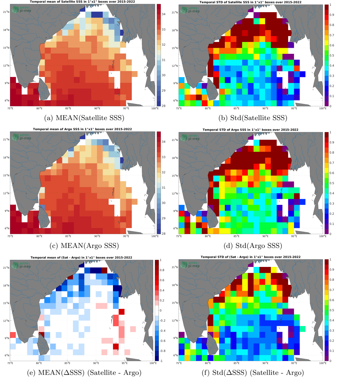
Figure 6: Temporal mean (left) and Std (right) of SSS from SMAP SSS L3 v5 - Monthly (RSS) (top), Argo (middle), and of \Delta SSS (Satellite - Argo). Only match-up pairs are used to generate these maps.
