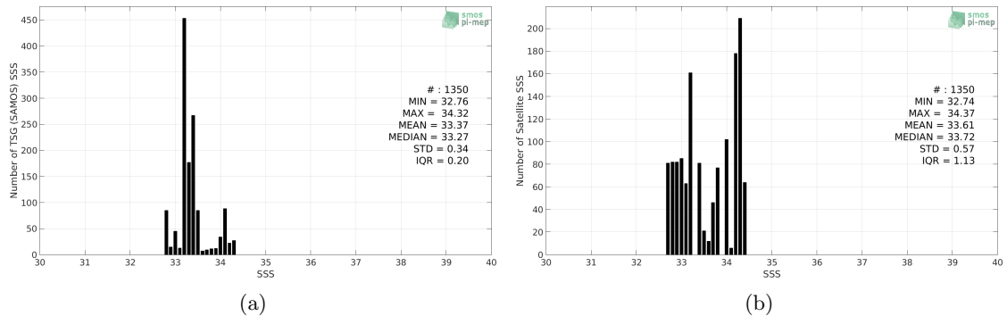
Figure 2: Histograms of SSS from TSG (SAMOS) (a) and SMAP SSS L3 v4 - 8-Day running (RSS) (b) considering all match-up pairs per bins of 0.1 over the Ganga and Brahmaputra river plumes Pi-MEP region and for the full satellite product period.
