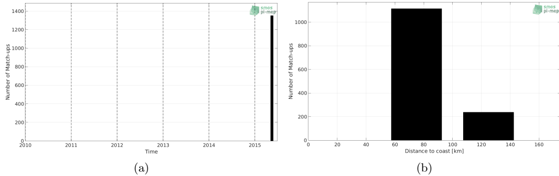
Figure 1: Number of match-ups between TSG (SAMOS) and SMAP SSS L3 v4 - 8-Day running (RSS) SSS as a function of time (a) and as function of the distance to coast (b) over the Ganga and Brahmaputra river plumes Pi-MEP region and for the full satellite product period.
