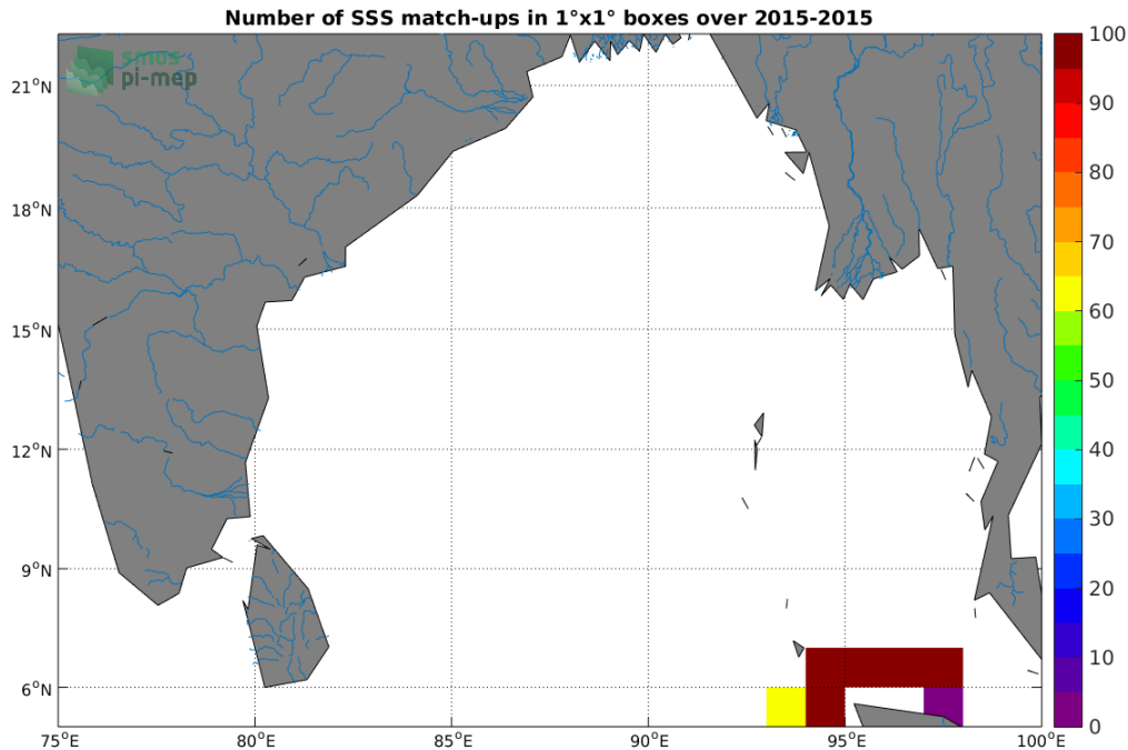
Figure 4: Number of SSS match-ups between TSG (SAMOS) SSS and the SMAP SSS L3 v4 - 8-Day running (RSS) SSS product for the Ganga and Brahmaputra river plumes Pi-MEP region over 1^\circ \times 1^\circ boxes and for the full satellite product period.
