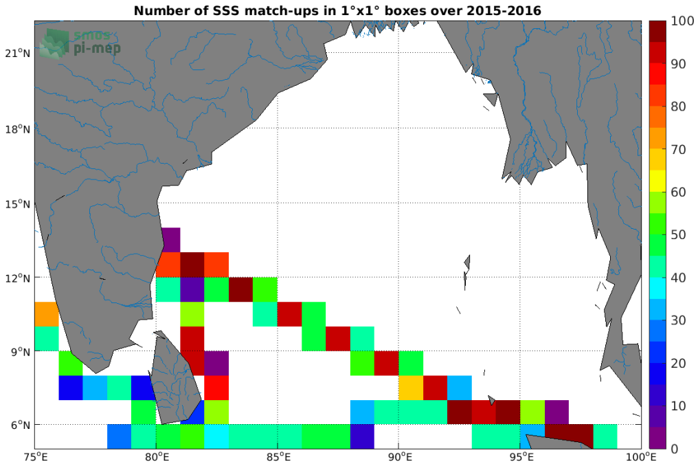
Figure 4: Number of SSS match-ups between TSG (LEGOS-DM) SSS and the SMAP SSS L3 v4 - 8-Day running (RSS) SSS product for the Ganga and Brahmaputra river plumes Pi-MEP region over 1°x1° boxes and for the full satellite product period.
