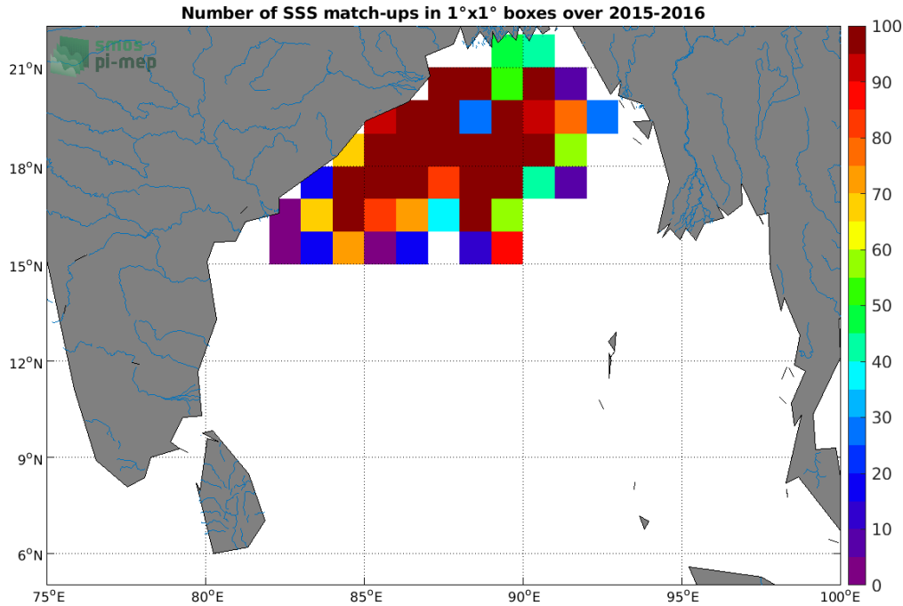
Figure 3: Number of SSS match-ups between Surface drifters SSS and the SMAP SSS L3 v4 - 8-Day running (RSS) SSS product for the Ganga and Brahmaputra river plumes Pi-MEP region over 1°x1° boxes and for the full satellite product period.
