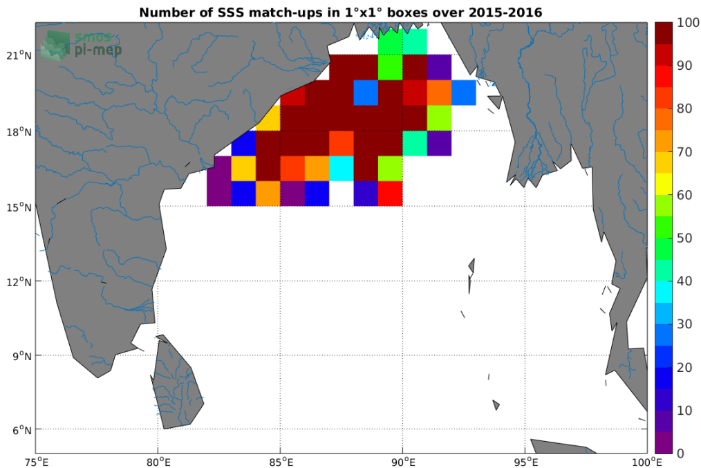
Figure 3: Number of SSS match-ups between Surface drifters SSS and the SMAP-L3-RSS-V4-8DAY-RUNNING SSS product for the Ganga and Brahmaputra river plumes Pi-MEP region over 1°x1° boxes and for the full satellite product period.
