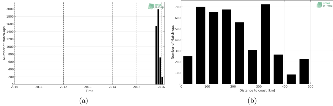
Figure 1: Number of match-ups between Surface drifters and SMAP-L3-RSS-V4-8DAY-RUNNING SSS as a function of time (a) and as function of the distance to coast (b) over the Ganga and Brahmaputra river plumes Pi-MEP region and for the full satellite product period.
