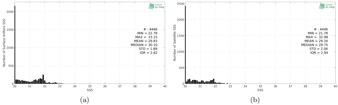
Figure 2: Histograms of SSS from Surface drifters (a) and SMAP-L3-RSS-V4-8DAY-RUNNING (b) considering all match-up pairs per bins of 0.1 over the Ganga and Brahmaputra river plumes Pi-MEP region and for the full satellite product period.
