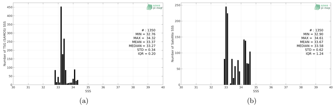
Figure 2: Histograms of SSS from TSG (SAMOS) (a) and SMAP SSS L3 v4 - Monthly (RSS) (b) considering all match-up pairs per bins of 0.1 over the Ganga and Brahmaputra river plumes Pi-MEP region and for the full satellite product period.
