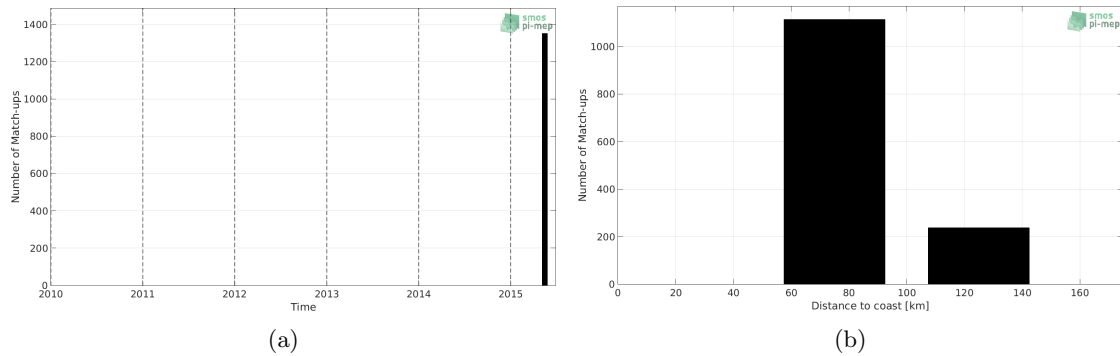
Figure 1: Number of match-ups between TSG (SAMOS) and SMAP SSS L3 v4 - Monthly (RSS) SSS as a function of time (a) and as function of the distance to coast (b) over the Ganga and Brahmaputra river plumes Pi-MEP region and for the full satellite product period.
