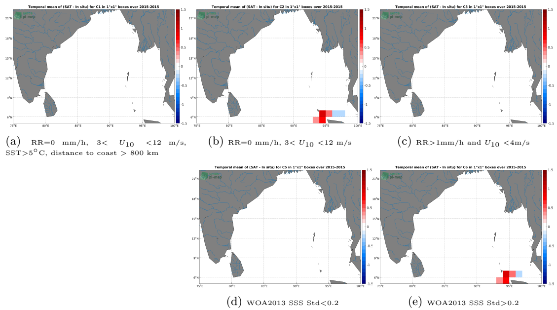
Figure 12: Temporal mean gridded over spatial boxes of size 1°x1° of \Delta SSS (SMAP SSS L3 v4 - Monthly (RSS) - TSG (SAMOS)) for 5 different subdatasets corresponding to:RR=0 mm/h, 3 < U_{10} < 12 m/s, SST>5°C, distance to coast > 800 km (a), RR=0 mm/h, 3 < U_{10} < 12 m/s (b), RR>1mm/h and U_{10} < 4 m/s (c), WOA2013 SSS Std<0.2 (d), WOA2013 SSS Std>0.2 (e).
