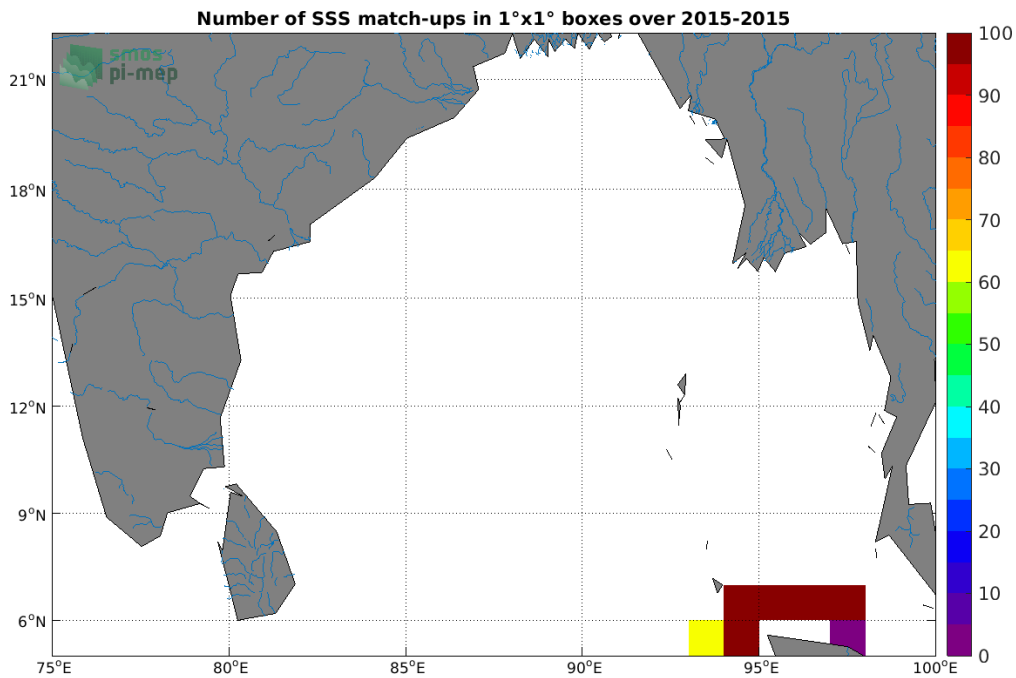
Figure 4: Number of SSS match-ups between TSG (SAMOS) SSS and the SMAP SSS L3 v4 - Monthly (RSS) SSS product for the Ganga and Brahmaputra river plumes Pi-MEP region over 1°x1° boxes and for the full satellite product period.
