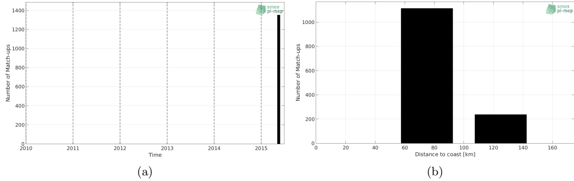
Figure 1: Number of match-ups between TSG-SAMOS and SMAP-L3-RSS-V4-MONTHLY SSS as a function of time (a) and as function of the distance to coast (b) over the Ganga and Brahmaputra river plumes Pi-MEP region and for the full satellite product period.
