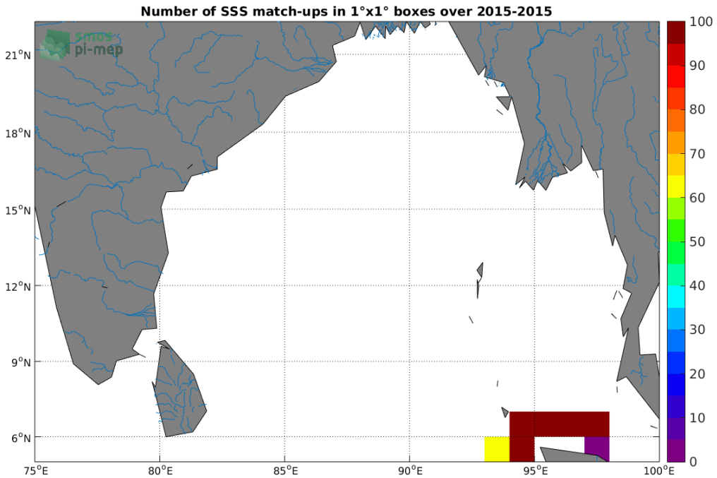
Figure 4: Number of SSS match-ups between TSG-SAMOS SSS and the SMAP-L3-RSS-V4-MONTHLY SSS product for the Ganga and Brahmaputra river plumes Pi-MEP region over 1^\circ \times 1^\circ boxes and for the full satellite product period.
