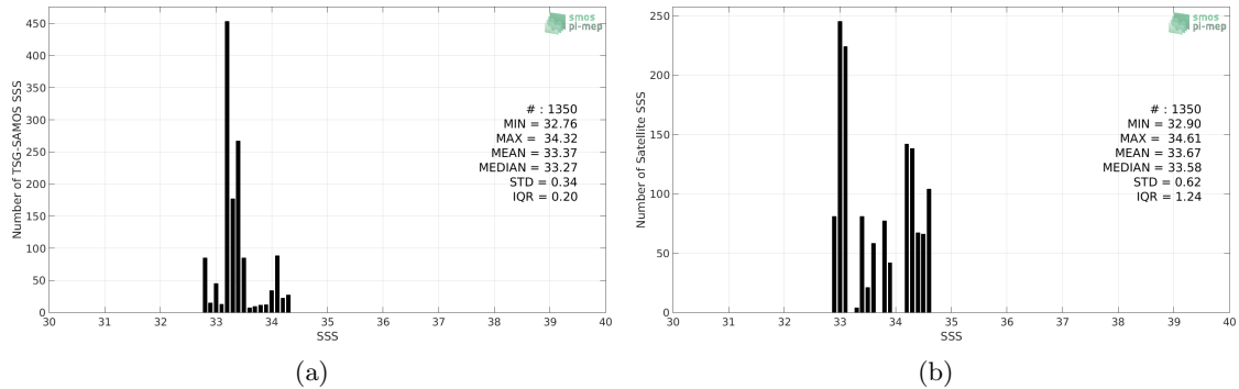
Figure 2: Histograms of SSS from TSG-SAMOS (a) and SMAP-L3-RSS-V4-MONTHLY (b) considering all match-up pairs per bins of 0.1 over the Ganga and Brahmaputra river plumes Pi-MEP region and for the full satellite product period.
