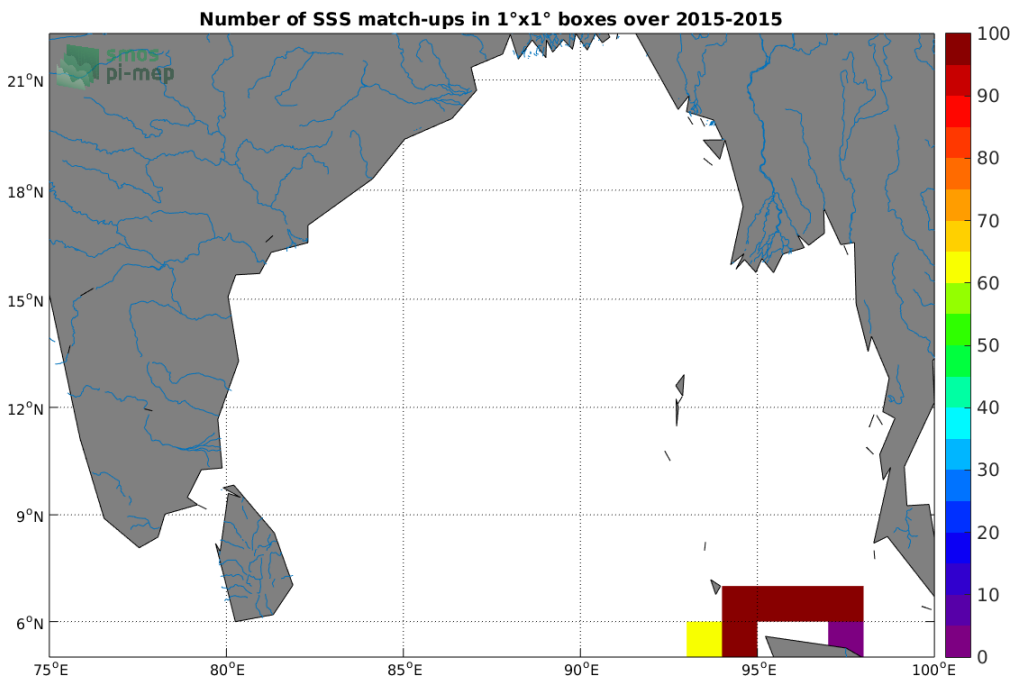
Figure 4: Number of SSS match-ups between TSG-SAMOS SSS and the SMAP-L3-RSS-V4-MONTHLY SSS product for the Ganga and Brahmaputra river plumes Pi-MEP region over 1°x1° boxes and for the full satellite product period.
