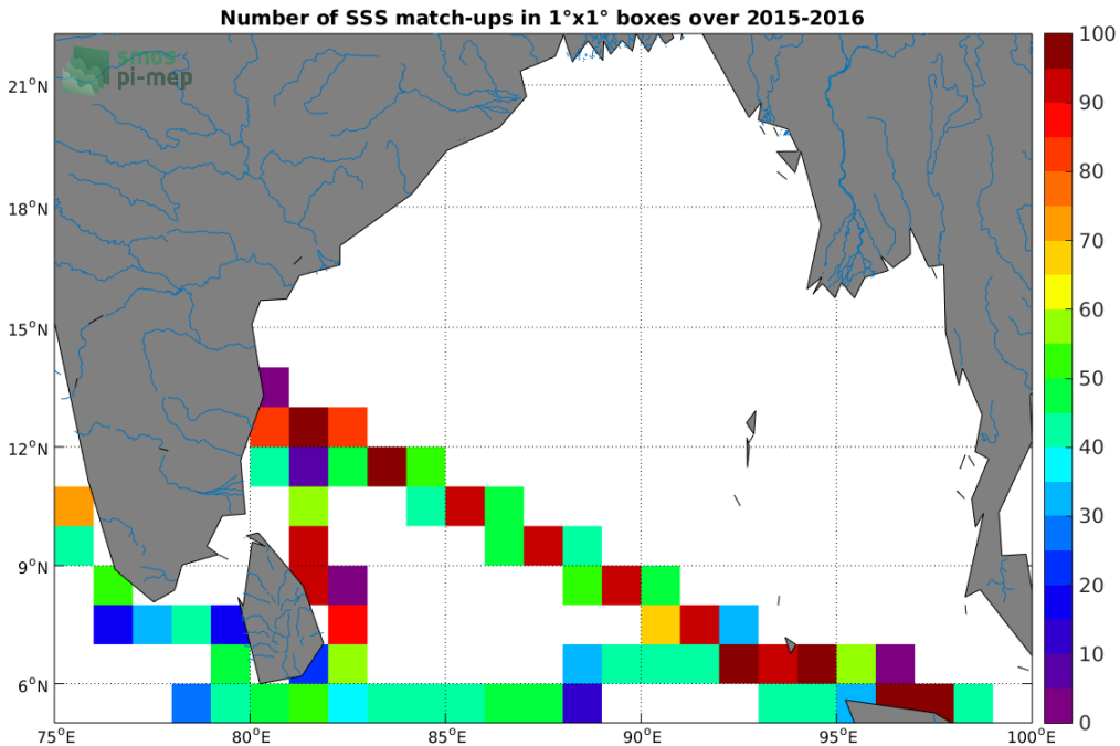
Figure 4: Number of SSS match-ups between TSG-LEGOS-DM SSS and the SMAP-L3-RSS-V4-MONTHLY SSS product for the Ganga and Brahmaputra river plumes Pi-MEP region over 1°x1° boxes and for the full satellite product period.
