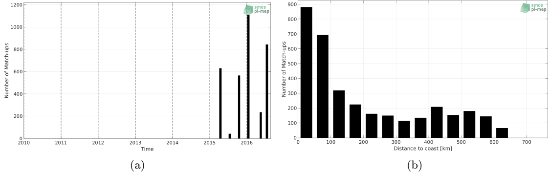
Figure 1: Number of match-ups between TSG-LEGOS-DM and SMAP-L3-RSS-V4-MONTHLY SSS as a function of time (a) and as function of the distance to coast (b) over the Ganga and Brahmaputra river plumes Pi-MEP region and for the full satellite product period.
