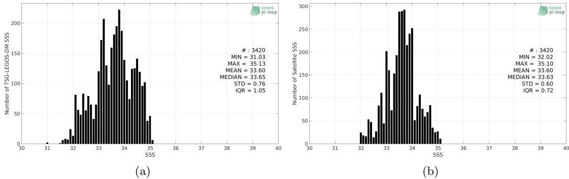
Figure 2: Histograms of SSS from TSG-LEGOS-DM (a) and SMAP-L3-RSS-V4-MONTHLY (b) considering all match-up pairs per bins of 0.1 over the Ganga and Brahmaputra river plumes Pi-MEP region and for the full satellite product period.
