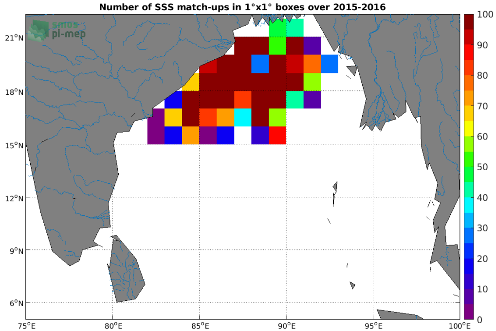
Figure 3: Number of SSS match-ups between Surface drifters SSS and the SMAP SSS L3 v4 - Monthly (RSS) SSS product for the Ganga and Brahmaputra river plumes Pi-MEP region over 1^\circ \times 1^\circ boxes and for the full satellite product period.
