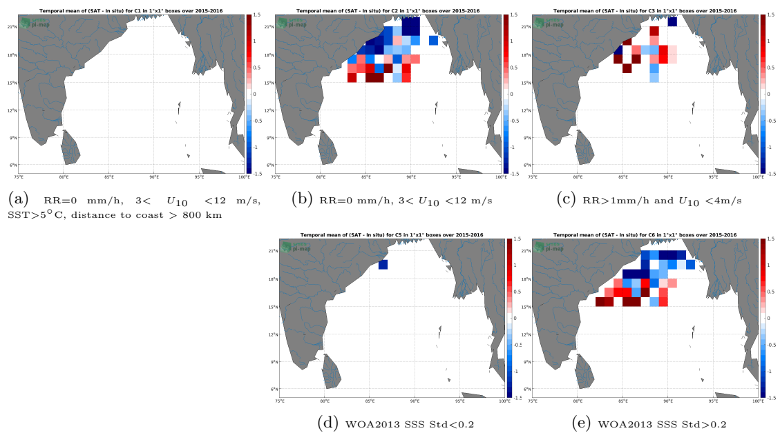
Figure 11: Temporal mean gridded over spatial boxes of size 1°x1° of \Delta SSS (SMAP SSS L3 v4 - Monthly (RSS) - Surface drifters) for 5 different subdatasets corresponding to:RR=0 mm/h, 3 < U_{10} < 12 m/s, SST>5°C, distance to coast > 800 km (a), RR=0 mm/h, 3 < U_{10} < 12 m/s (b), RR>1mm/h and U_{10} < 4 m/s (c), WOA2013 SSS Std<0.2 (d), WOA2013 SSS Std>0.2 (e).
