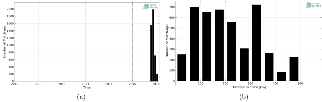
Figure 1: Number of match-ups between Surface drifters and SMAP SSS L3 v4 - Monthly (RSS) SSS as a function of time (a) and as function of the distance to coast (b) over the Ganga and Brahmaputra river plumes Pi-MEP region and for the full satellite product period.
