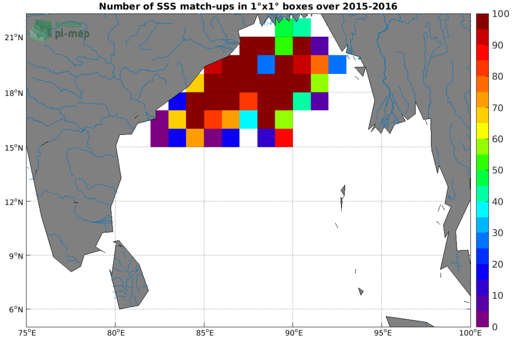
Figure 3: Number of SSS match-ups between Surface drifters SSS and the SMAP SSS L3 v4 - Monthly (RSS) SSS product for the Ganga and Brahmaputra river plumes Pi-MEP region over 1°x1° boxes and for the full satellite product period.
