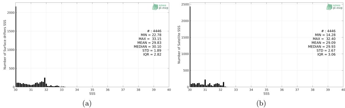
Figure 2: Histograms of SSS from Surface drifters (a) and SMAP SSS L3 v4 - Monthly (RSS) (b) considering all match-up pairs per bins of 0.1 over the Ganga and Brahmaputra river plumes Pi-MEP region and for the full satellite product period.
