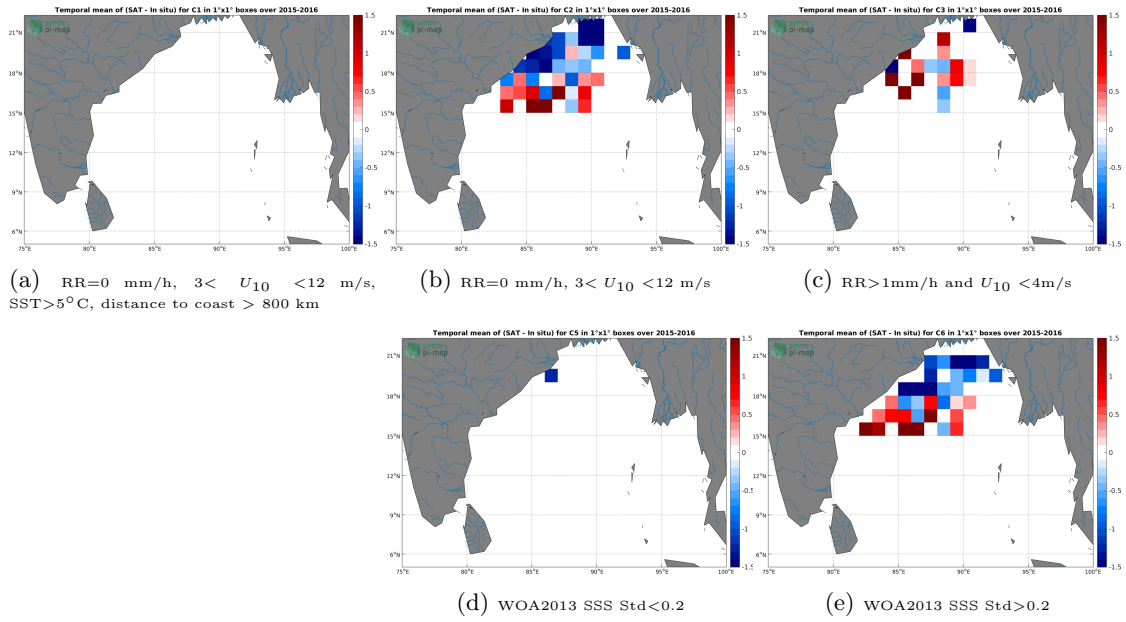
Figure 11: Temporal mean gridded over spatial boxes of size 1^\circ \times 1^\circ of \Delta SSS (SMAP-L3-RSS-V4-MONTHLY - Surface drifters) for 5 different subdatasets corresponding to:RR=0 mm/h, 3 < U_{10} < 12 m/s, SST >5^\circ C, distance to coast > 800 km (a), RR=0 mm/h, 3 < U_{10} < 12 m/s (b), RR >1 mm/h and U_{10} < 4 m/s (c), WOA2013 SSS Std <0.2 (d), WOA2013 SSS Std >0.2 (e).
