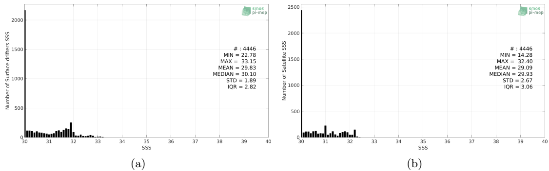
Figure 2: Histograms of SSS from Surface drifters (a) and SMAP-L3-RSS-V4-MONTHLY (b) considering all match-up pairs per bins of 0.1 over the Ganga and Brahmaputra river plumes Pi-MEP region and for the full satellite product period.
