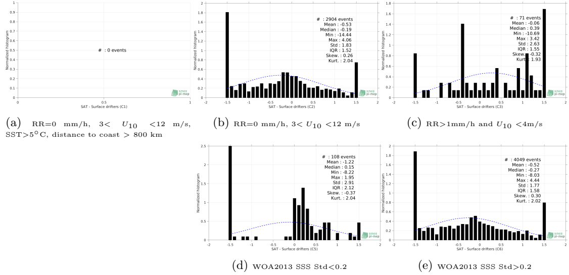
Figure 12: Normalized histogram of \Delta SSS (SMAP-L3-RSS-V4-MONTHLY - Surface drifters) for 5 different subdatasets corresponding to: RR=0 mm/h, 3 < U_{10} < 12 m/s, SST > 5°C, distance to coast > 800 km (a), RR=0 mm/h, 3 < U_{10} < 12 m/s (b), RR > 1mm/h and U_{10} < 4 m/s (c), WOA2013 SSS Std < 0.2 (d), WOA2013 SSS Std > 0.2 (e).
