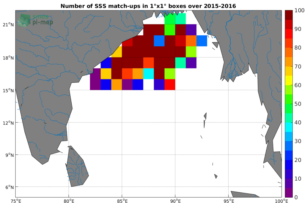
Figure 3: Number of SSS match-ups between Surface drifters SSS and the SMAP-L3-RSS-V4-MONTHLY SSS product for the Ganga and Brahmaputra river plumes Pi-MEP region over 1°x1° boxes and for the full satellite product period.
