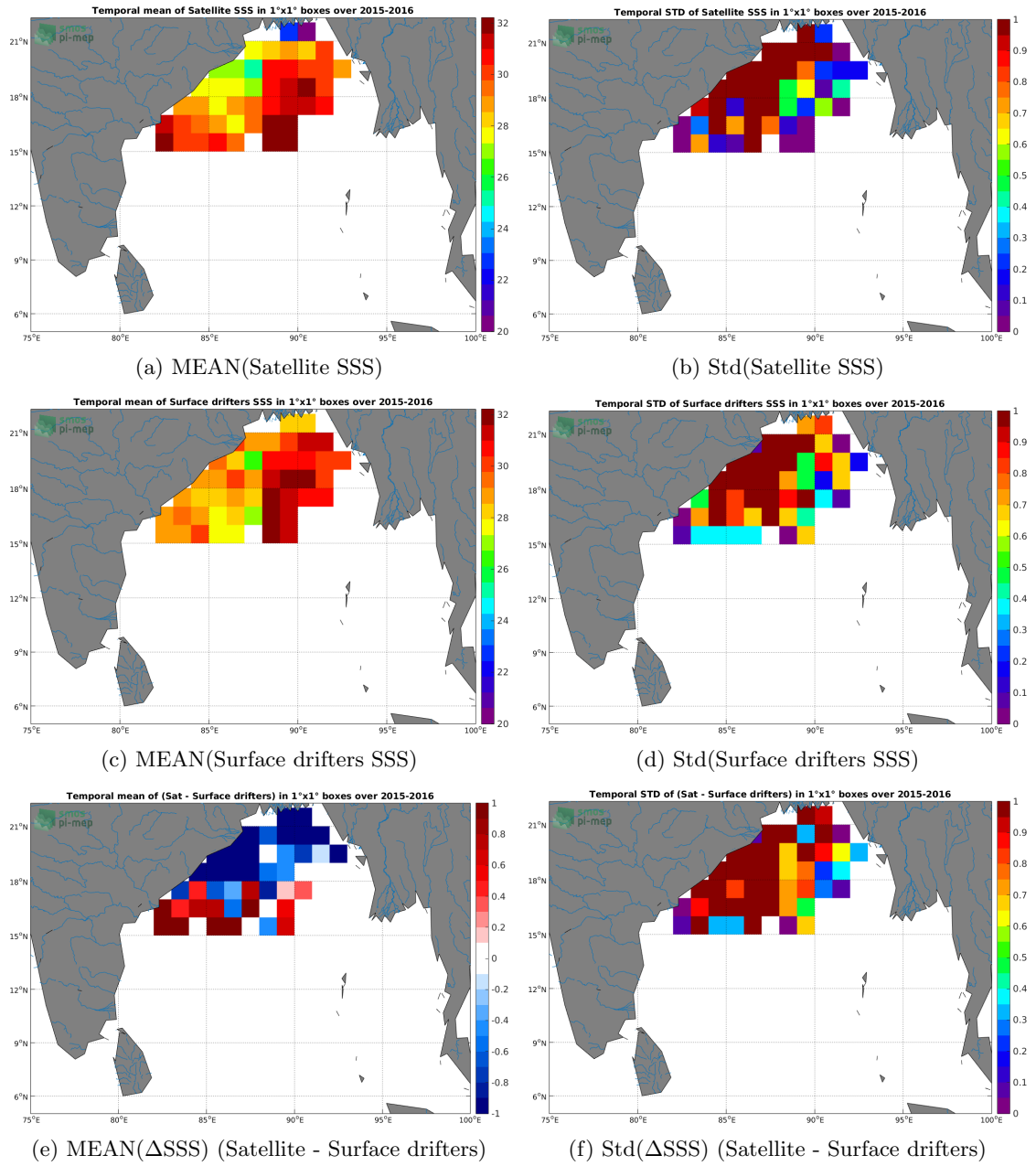
Figure 5: Temporal mean (left) and Std (right) of SSS from SMAP-L3-RSS-V4-MONTHLY (top), Surface drifters (middle), and of \Delta SSS (Satellite - Surface drifters). Only match-up pairs are used to generate these maps.
