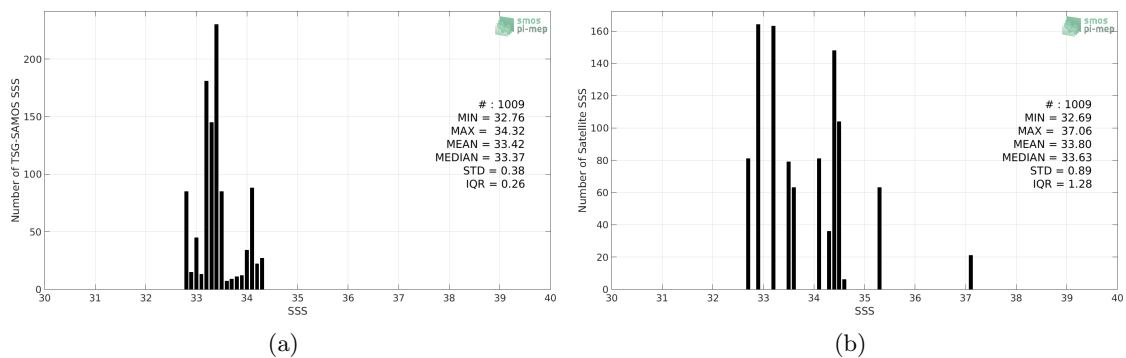
Figure 2: Histograms of SSS from TSG-SAMOS (a) and SMAP-L3-RSS-V3-8DAY-RUNNING-40KM (b) considering all match-up pairs per bins of 0.1 over the Ganga and Brahmaputra river plumes Pi-MEP region and for the full satellite product period.
