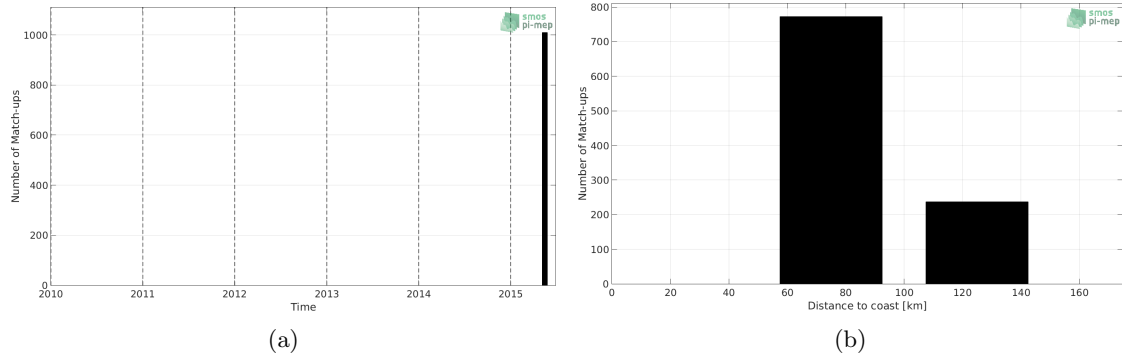
Figure 1: Number of match-ups between TSG-SAMOS and SMAP-L3-RSS-V3-8DAY-RUNNING-40KM SSS as a function of time (a) and as function of the distance to coast (b) over the Ganga and Brahmaputra river plumes Pi-MEP region and for the full satellite product period.
