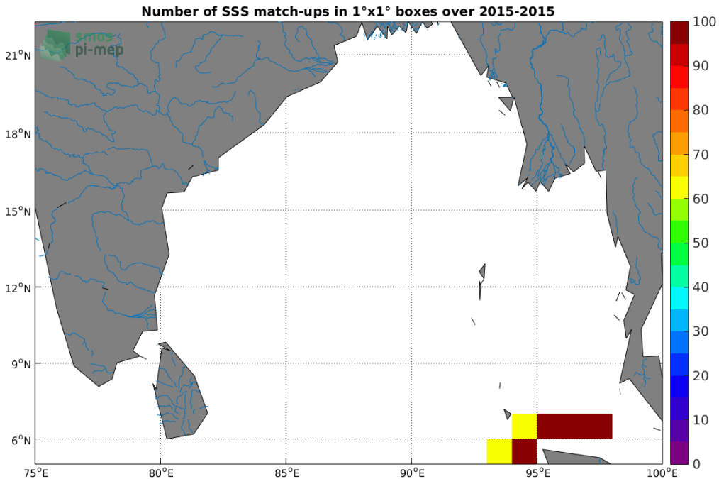
Figure 4: Number of SSS match-ups between TSG-SAMOS SSS and the SMAP-L3-RSS-V3-8DAY-RUNNING-40KM SSS product for the Ganga and Brahmaputra river plumes Pi-MEP region over 1^{\circ} \times 1^{\circ} boxes and for the full satellite product period.
