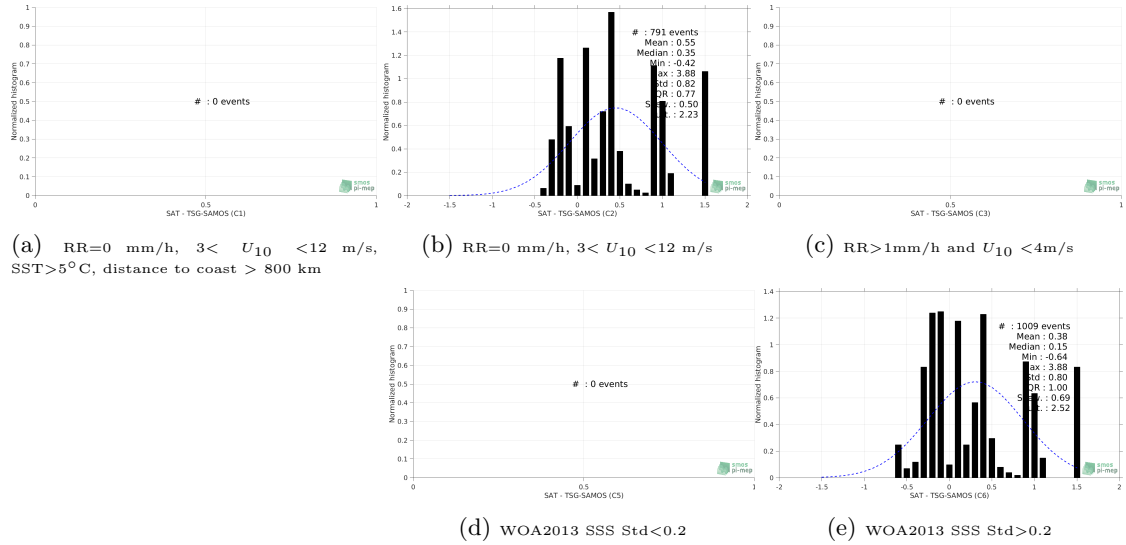
Figure 13: Normalized histogram of \Delta SSS (SMAP-L3-RSS-V3-8DAY-RUNNING-40KM - TSG-SAMOS) for 5 different subdatasets corresponding to: RR=0 mm/h, 3 < U_{10} < 12 m/s, SST >5^{\circ} C, distance to coast > 800 km (a), RR=0 mm/h, 3 < U_{10} < 12 m/s (b), RR >1 mm/h and U_{10} < 4 m/s (c), WOA2013 SSS Std <0.2 (d), WOA2013 SSS Std >0.2 (e).
