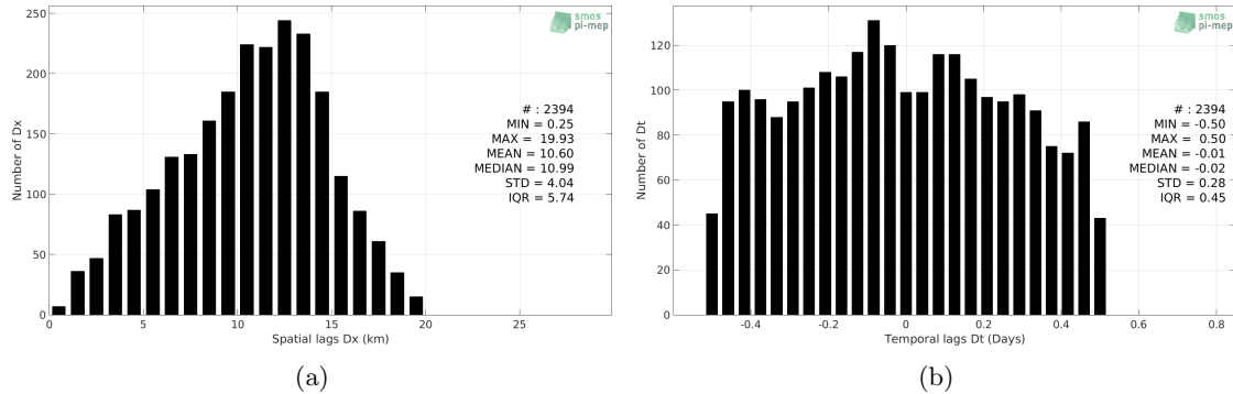
Figure 5: Histograms of the spatial (a) and temporal (b) lags between the time of the TSG-LEGOS-DM measurements and the date of the corresponding SMAP-L3-RSS-V3-8DAY-RUNNING-40KM SSS product.
