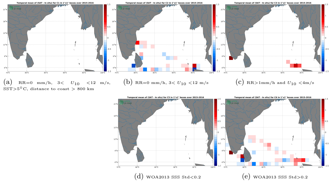
Figure 12: Temporal mean gridded over spatial boxes of size 1^\circ \times 1^\circ of \Delta SSS (SMAP-L3-RSS-V3-8DAY-RUNNING-40KM - TSG-LEGOS-DM) for 5 different subdatasets corresponding to:RR=0 mm/h, 3 < U_{10} < 12 m/s, SST >5^\circ C, distance to coast > 800 km (a), RR=0 mm/h, 3 < U_{10} < 12 m/s (b), RR >1 mm/h and U_{10} < 4 m/s (c), WOA2013 SSS Std <0.2 (d), WOA2013 SSS Std >0.2 (e).
