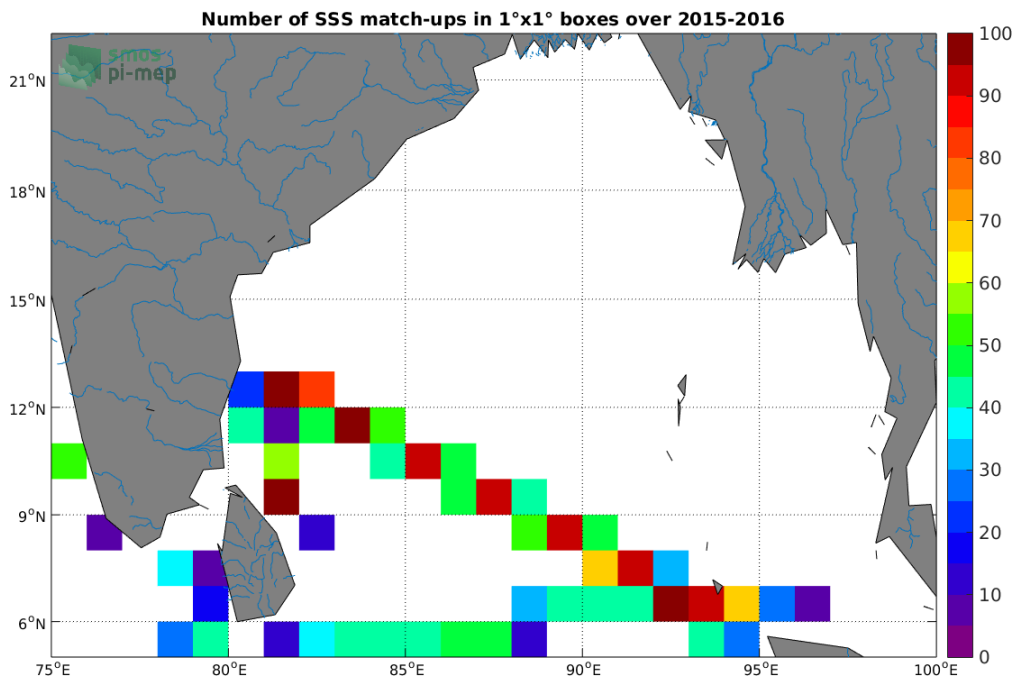
Figure 4: Number of SSS match-ups between TSG-LEGOS-DM SSS and the SMAP-L3-RSS-V3-8DAY-RUNNING-40KM SSS product for the Ganga and Brahmaputra river plumes Pi-MEP region over 1^{\circ} \times 1^{\circ} boxes and for the full satellite product period.
