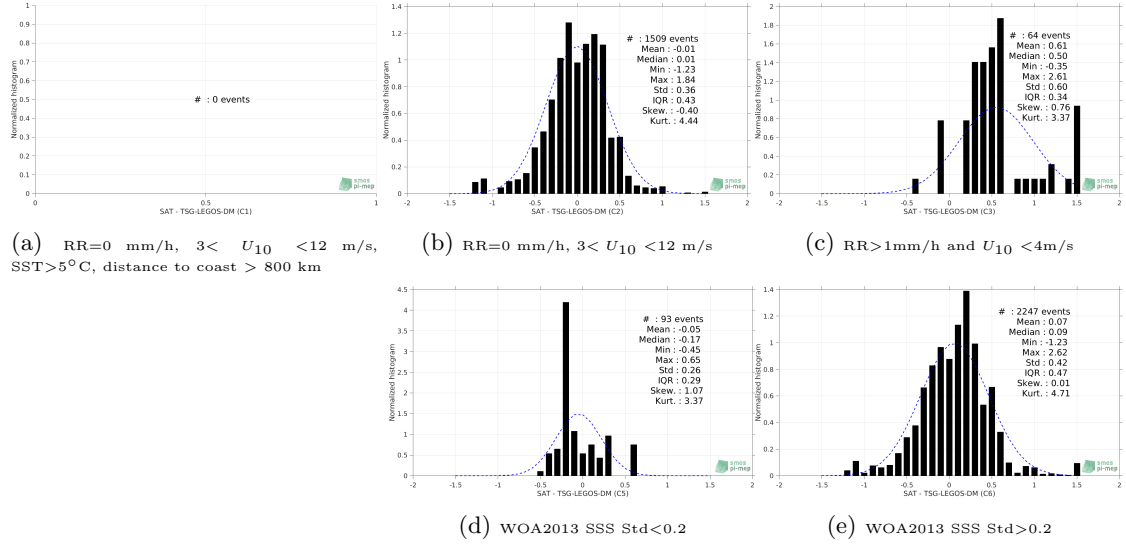
Figure 13: Normalized histogram of \Delta SSS (SMAP-L3-RSS-V3-8DAY-RUNNING-40KM - TSG-LEGOS-DM) for 5 different subdatasets corresponding to: RR=0 mm/h, 3 < U_{10} < 12 m/s, SST > 5°C, distance to coast > 800 km (a), RR=0 mm/h, 3 < U_{10} < 12 m/s (b), RR > 1mm/h and U_{10} < 4 m/s (c), WOA2013 SSS Std < 0.2 (d), WOA2013 SSS Std > 0.2 (e).
