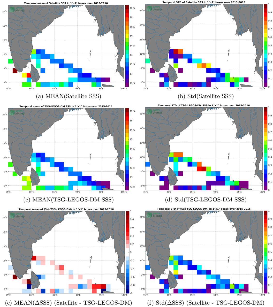
Figure 6: Temporal mean (left) and Std (right) of SSS from SMAP-L3-RSS-V3-8DAY-RUNNING-40KM (top), TSG-LEGOS-DM (middle), and of \Delta SSS (Satellite - TSG-LEGOS-DM). Only match-up pairs are used to generate these maps.
