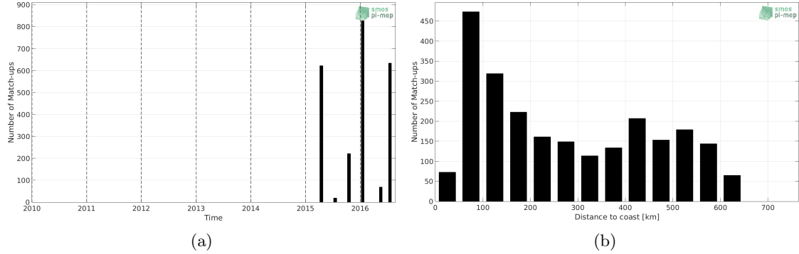
Figure 1: Number of match-ups between TSG-LEGOS-DM and SMAP-L3-RSS-V3-8DAY-RUNNING-40KM SSS as a function of time (a) and as function of the distance to coast (b) over the Ganga and Brahmaputra river plumes Pi-MEP region and for the full satellite product period.
