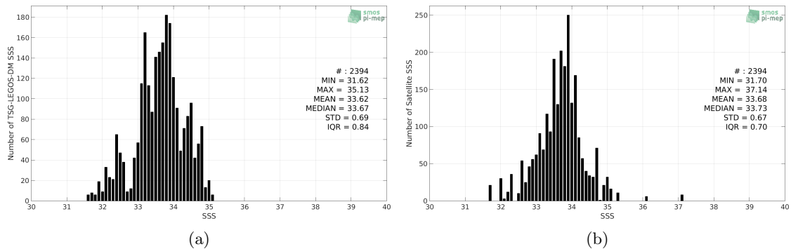
Figure 2: Histograms of SSS from TSG-LEGOS-DM (a) and SMAP-L3-RSS-V3-8DAY-RUNNING-40KM (b) considering all match-up pairs per bins of 0.1 over the Ganga and Brahmaputra river plumes Pi-MEP region and for the full satellite product period.
