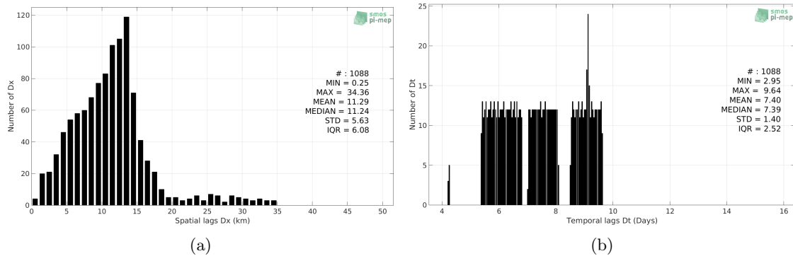
Figure 5: Histograms of the spatial (a) and temporal (b) lags between the time of the TSG-LEGOS-DM measurements and the date of the corresponding SMAP-L3-RSS-V3-MONTHLY-70KM SSS product.
