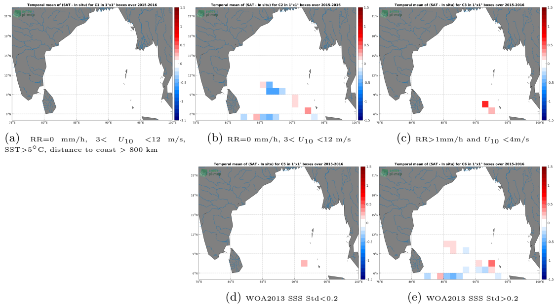
Figure 12: Temporal mean gridded over spatial boxes of size 1^\circ \times 1^\circ of \Delta SSS (SMAP-L3-RSS-V3-MONTHLY-70KM - TSG-LEGOS-DM) for 5 different subdatasets corresponding to:RR=0 mm/h, 3 < U_{10} < 12 m/s, SST >5^\circ C, distance to coast > 800 km (a), RR=0 mm/h, 3 < U_{10} < 12 m/s (b), RR >1 mm/h and U_{10} < 4 m/s (c), WOA2013 SSS Std <0.2 (d), WOA2013 SSS Std >0.2 (e).
