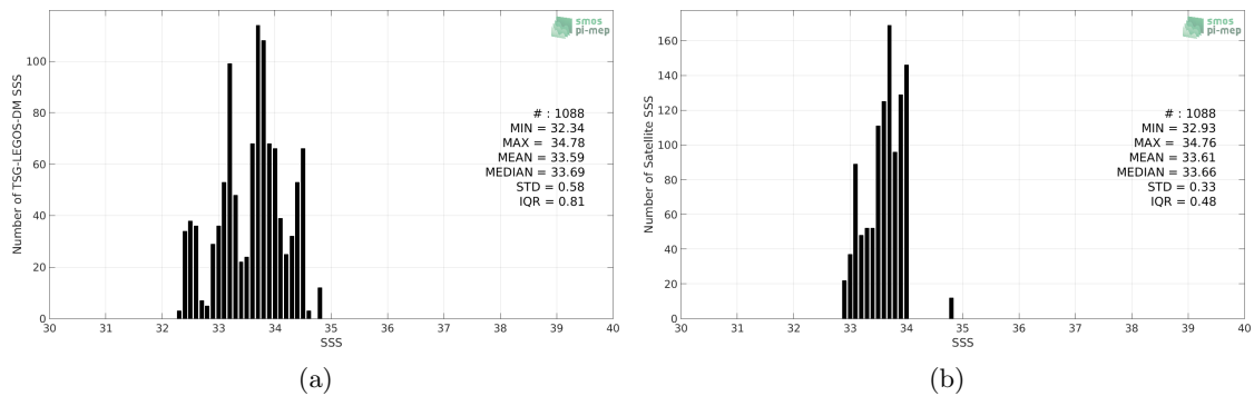
Figure 2: Histograms of SSS from TSG-LEGOS-DM (a) and SMAP-L3-RSS-V3-MONTHLY-70KM (b) considering all match-up pairs per bins of 0.1 over the Ganga and Brahmaputra river plumes Pi-MEP region and for the full satellite product period.
