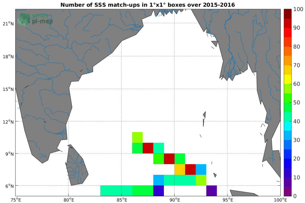
Figure 4: Number of SSS match-ups between TSG-LEGOS-DM SSS and the SMAP-L3-RSS-V3-MONTHLY-70KM SSS product for the Ganga and Brahmaputra river plumes Pi-MEP region over 1^{\circ} \times 1^{\circ} boxes and for the full satellite product period.
