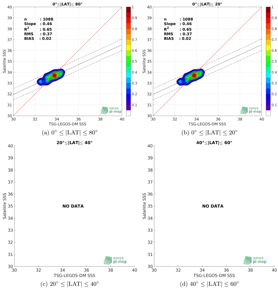
Figure 9: Contour maps of the concentration of SMAP-L3-RSS-V3-MONTHLY-70KM SSS (y-axis) versus TSG-LEGOS-DM SSS (x-axis) at match-up pairs for different latitude bands. For each plot, the red line shows x=y . The black thin and dashed lines indicate a linear fit through the data cloud and the \pm 95\% confidence levels, respectively. The number match-up pairs n , the slope and R^2 coefficient of the linear fit, the root mean square (RMS) and the mean bias between satellite and in situ data are indicated for each latitude band in each plots.
