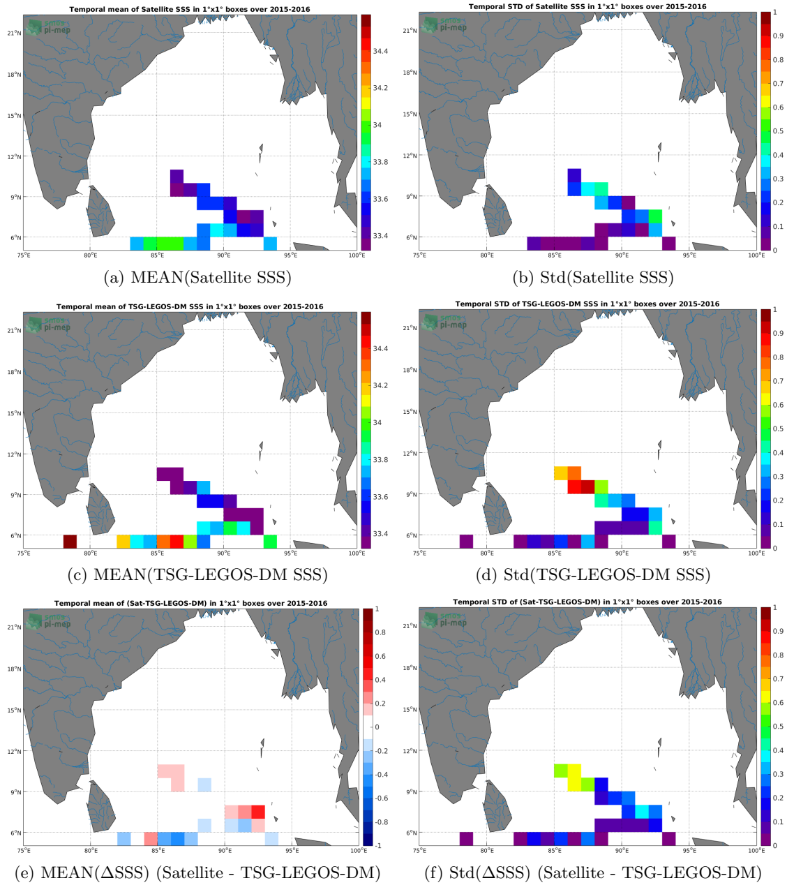
Figure 6: Temporal mean (left) and Std (right) of SSS from SMAP-L3-RSS-V3-MONTHLY-70KM (top), TSG-LEGOS-DM (middle), and of \Delta SSS (Satellite - TSG-LEGOS-DM). Only match-up pairs are used to generate these maps.
