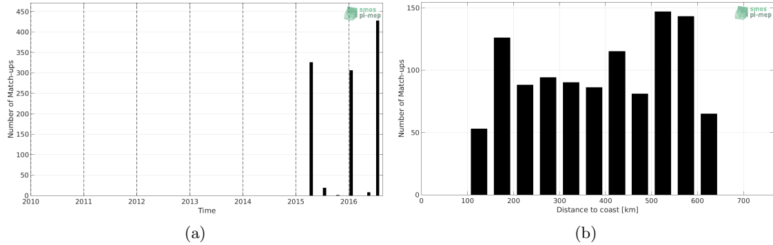
Figure 1: Number of match-ups between TSG-LEGOS-DM and SMAP-L3-RSS-V3-MONTHLY-70KM SSS as a function of time (a) and as function of the distance to coast (b) over the Ganga and Brahmaputra river plumes Pi-MEP region and for the full satellite product period.
