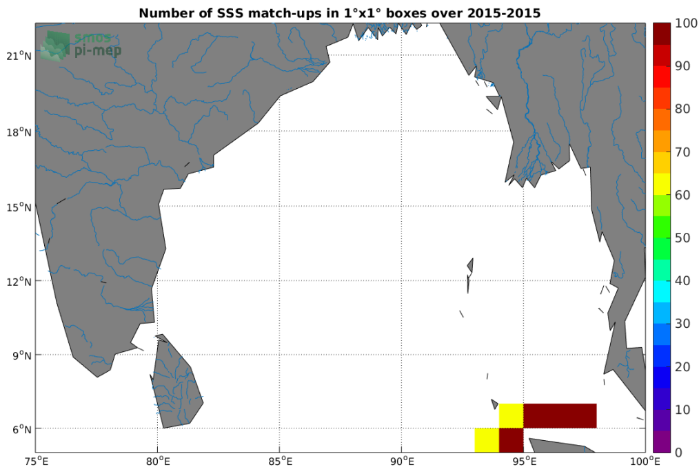
Figure 4: Number of SSS match-ups between TSG-SAMOS SSS and the SMAP-L3-RSS-V3-MONTHLY-0.25DEG-40KM SSS product for the Ganga and Brahmaputra river plumes Pi-MEP region over 1°x1° boxes and for the full satellite product period.
