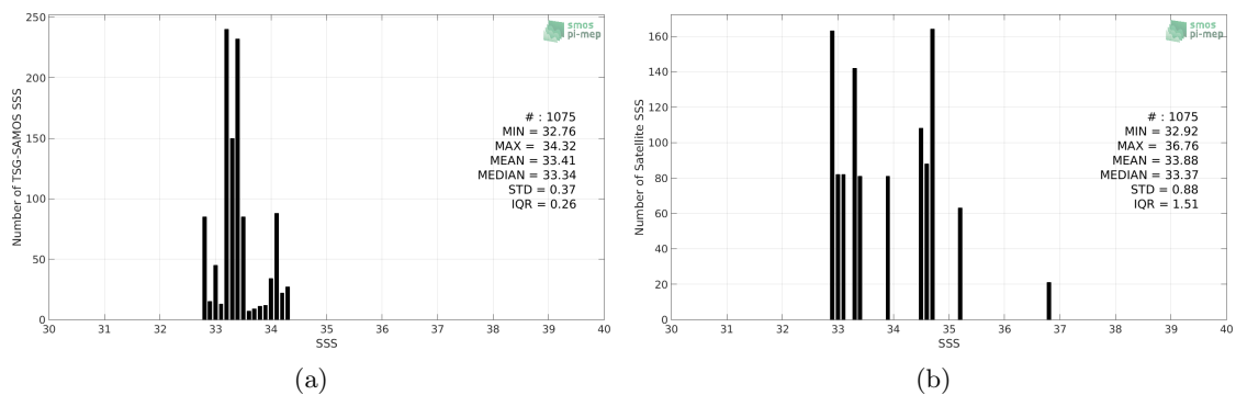
Figure 2: Histograms of SSS from TSG-SAMOS (a) and SMAP-L3-RSS-V3-MONTHLY-0.25DEG-40KM (b) considering all match-up pairs per bins of 0.1 over the Ganga and Brahmaputra river plumes Pi-MEP region and for the full satellite product period.
