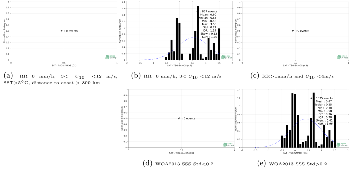
Figure 13: Normalized histogram of \Delta SSS (SMAP-L3-RSS-V3-MONTHLY-0.25DEG-40KM - TSG-SAMOS) for 5 different subdatasets corresponding to: RR=0 mm/h, 3 < U_{10} < 12 m/s, SST > 5°C, distance to coast > 800 km (a), RR=0 mm/h, 3 < U_{10} < 12 m/s (b), RR > 1mm/h and U_{10} < 4 m/s (c), WOA2013 SSS Std < 0.2 (d), WOA2013 SSS Std > 0.2 (e).
