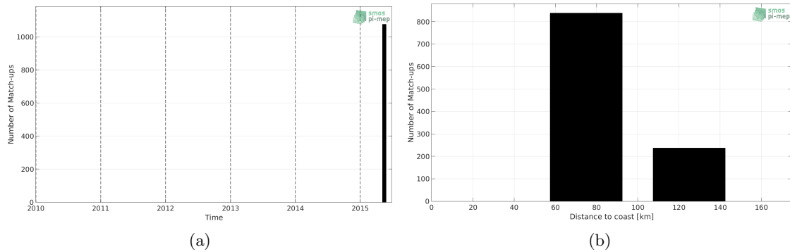
Figure 1: Number of match-ups between TSG-SAMOS and SMAP-L3-RSS-V3-MONTHLY-0.25DEG-40KM SSS as a function of time (a) and as function of the distance to coast (b) over the Ganga and Brahmaputra river plumes Pi-MEP region and for the full satellite product period.
