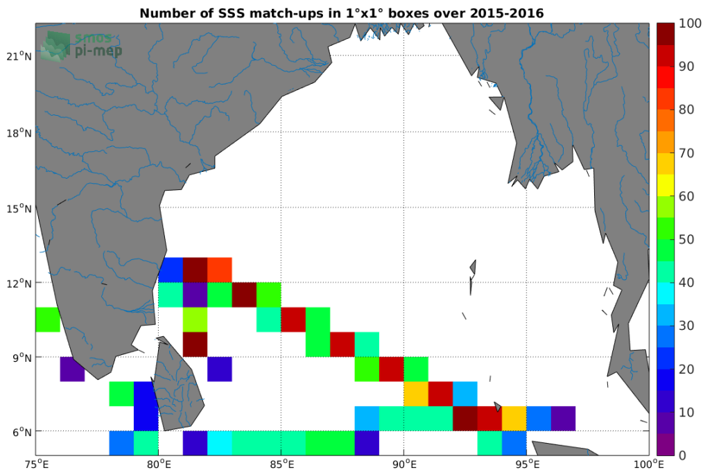
Figure 4: Number of SSS match-ups between TSG-LEGOS-DM SSS and the SMAP-L3-RSS-V3-MONTHLY-0.25DEG-40KM SSS product for the Ganga and Brahmaputra river plumes Pi-MEP region over 1^{\circ} \times 1^{\circ} boxes and for the full satellite product period.
