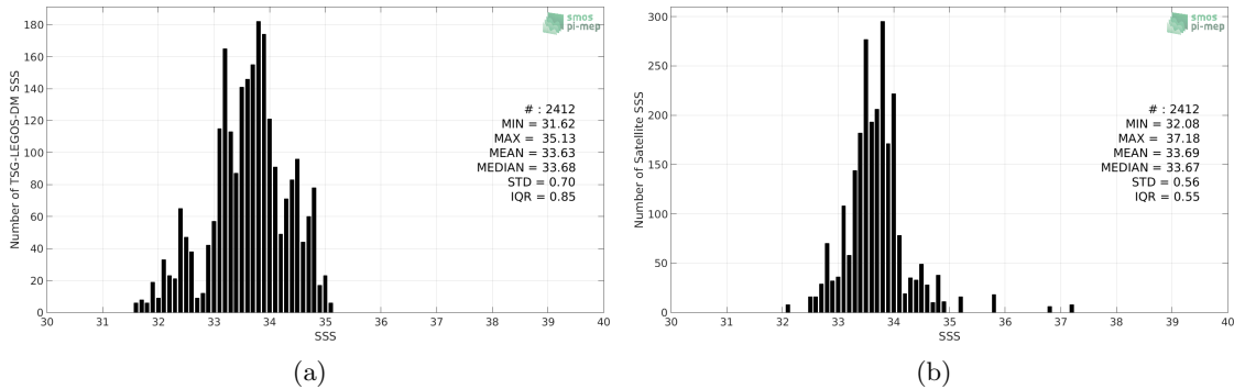
Figure 2: Histograms of SSS from TSG-LEGOS-DM (a) and SMAP-L3-RSS-V3-MONTHLY-0.25DEG-40KM (b) considering all match-up pairs per bins of 0.1 over the Ganga and Brahmaputra river plumes Pi-MEP region and for the full satellite product period.
