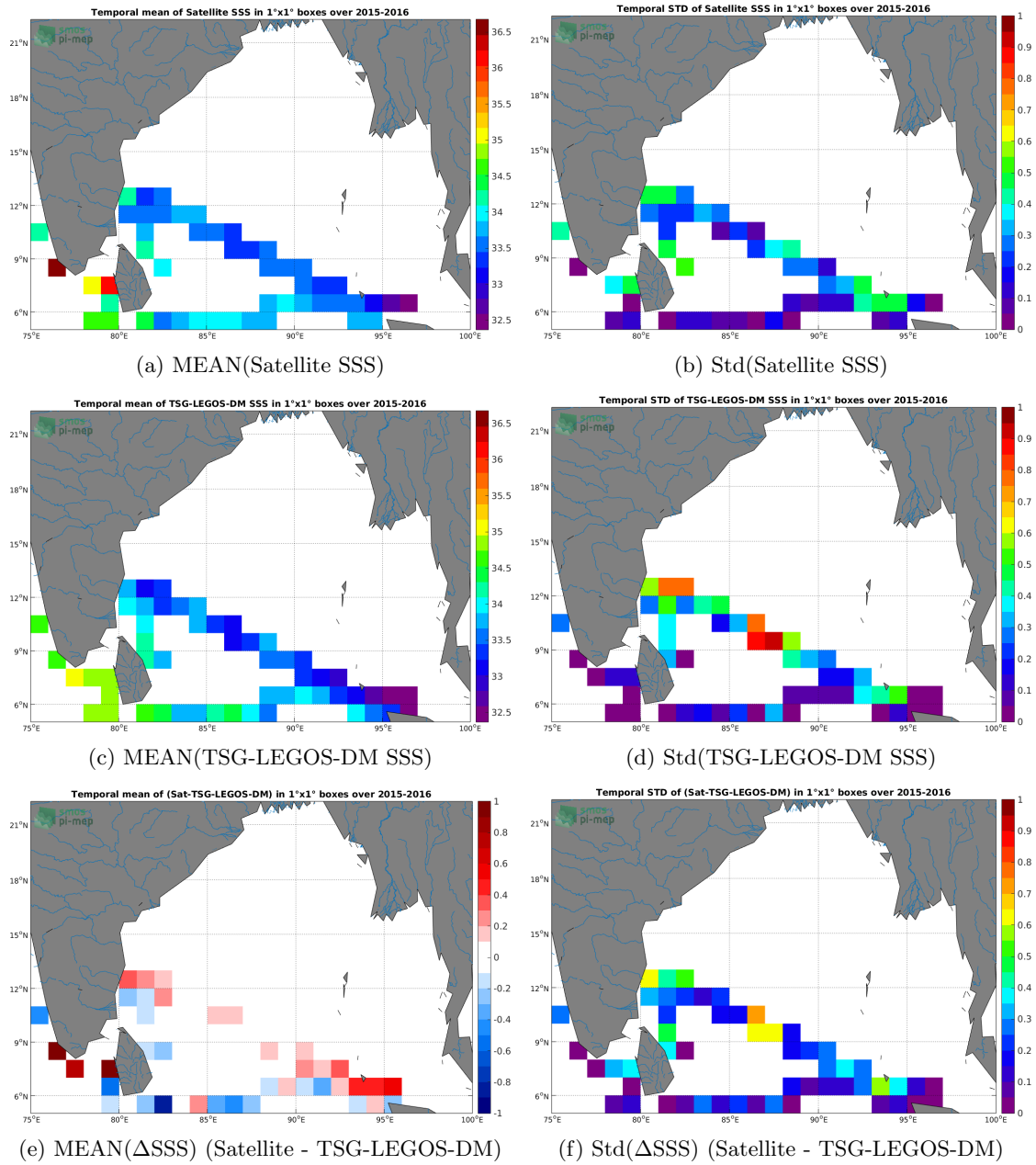
Figure 6: Temporal mean (left) and Std (right) of SSS from SMAP-L3-RSS-V3-MONTHLY-0.25DEG-40KM (top), TSG-LEGOS-DM (middle), and of \Delta SSS (Satellite - TSG-LEGOS-DM). Only match-up pairs are used to generate these maps.
