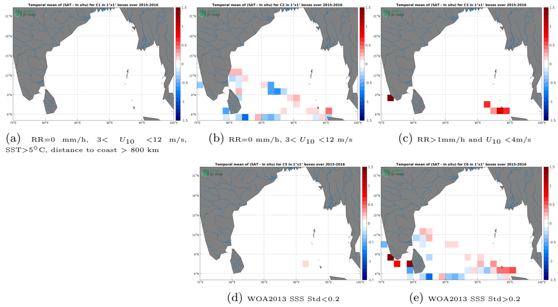
Figure 12: Temporal mean gridded over spatial boxes of size 1^\circ \times 1^\circ of \Delta SSS (SMAP-L3-RSS-V3-MONTHLY-0.25DEG-40KM - TSG-LEGOS-DM) for 5 different subdatasets corresponding to: RR=0 mm/h, 3 < U_{10} < 12 m/s, SST >5^\circ C, distance to coast > 800 km (a), RR=0 mm/h, 3 < U_{10} < 12 m/s (b), RR >1 mm/h and U_{10} < 4 m/s (c), WOA2013 SSS Std <0.2 (d), WOA2013 SSS Std >0.2 (e).
