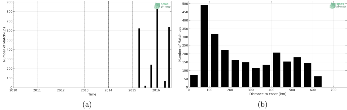
Figure 1: Number of match-ups between TSG-LEGOS-DM and SMAP-L3-RSS-V3-MONTHLY-0.25DEG-40KM SSS as a function of time (a) and as function of the distance to coast (b) over the Ganga and Brahmaputra river plumes Pi-MEP region and for the full satellite product period.
