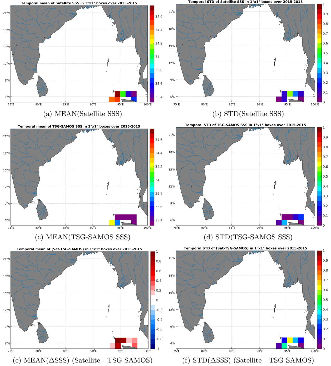
Figure 6: Temporal mean (left) and STD (right) of SSS from SMAP-L3-RSS-V2-8DAY-RUNNING-40KM (top), TSG-SAMOS (middle), and of \Delta SSS (Satellite - TSG-SAMOS). Only match-up pairs are used to generate these maps.
