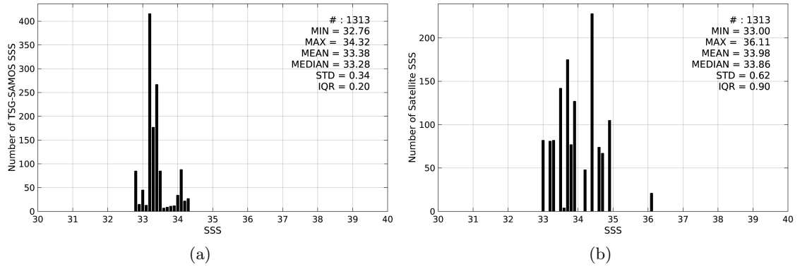
Figure 2: Histograms of SSS from TSG-SAMOS (a) and SMAP-L3-RSS-V2-8DAY-RUNNING-40KM (b) considering all match-up pairs per bins of 0.1 over the Ganga and Brahmaputra river plumes Pi-MEP region and for the full satellite product period.
