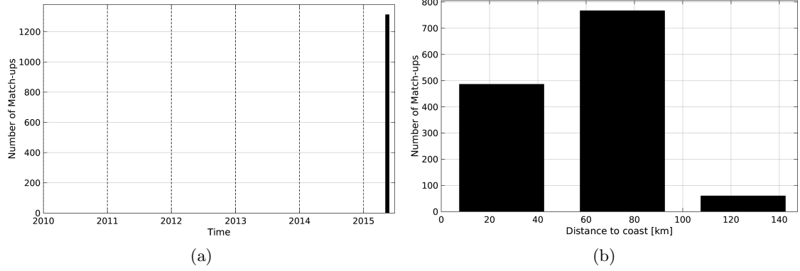
Figure 1: Number of match-ups between TSG-SAMOS and SMAP-L3-RSS-V2-8DAY-RUNNING-40KM SSS as a function of time (a) and as function of the distance to coast (b) over the Ganga and Brahmaputra river plumes Pi-MEP region and for the full satellite product period.
