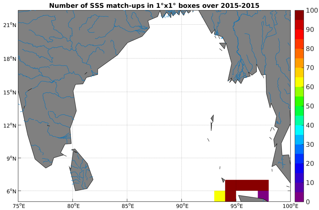
Figure 4: Number of SSS match-ups between TSG-SAMOS SSS and the SMAP-L3-RSS-V2-8DAY-RUNNING-40KM SSS product for the Ganga and Brahmaputra river plumes Pi-MEP region over 1^\circ \times 1^\circ boxes and for the full satellite product period.
