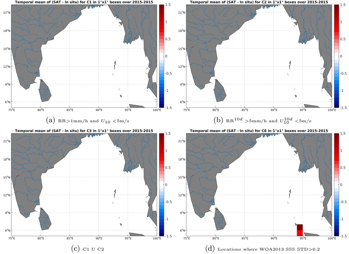
Figure 12: Temporal mean gridded over spatial boxes of size 1^\circ \times 1^\circ of \Delta SSS (SMAP-L3-RSS-V2-8DAY-RUNNING-40KM - TSG-SAMOS) for 4 different subdatasets corresponding to: RR > 1 mm/h and U_{10} < 5 m/s (a), RR^{10d} > 5 mm/h and U_{10}^{10d} < 5 m/s (b), C1 U C2 (c), Locations where WOA2013 SSS STD > 0.2 (d).
