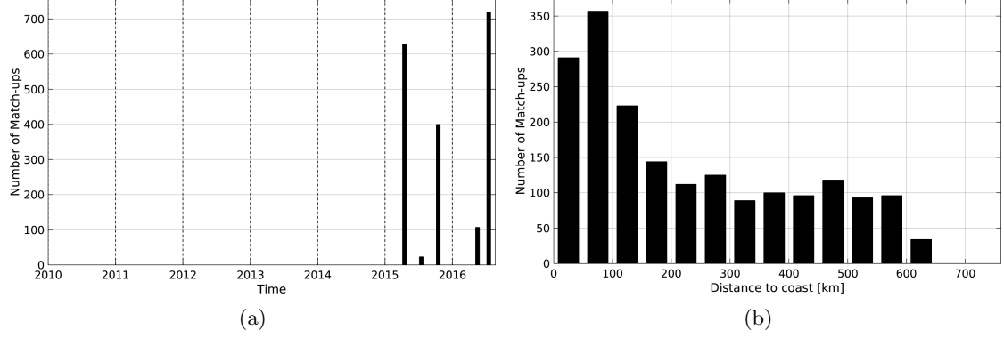
Figure 1: Number of match-ups between TSG-LEGOS-DM and SMAP-L3-RSS-V2-8DAY-RUNNING-40KM SSS as a function of time (a) and as function of the distance to coast (b) over the Ganga and Brahmaputra river plumes Pi-MEP region and for the full satellite product period.
