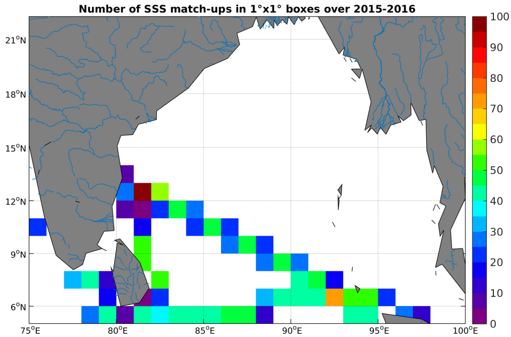
Figure 4: Number of SSS match-ups between TSG-LEGOS-DM SSS and the SMAP-L3-RSS-V2-8DAY-RUNNING-40KM SSS product for the Ganga and Brahmaputra river plumes Pi-MEP region over 1^\circ \times 1^\circ boxes and for the full satellite product period.
