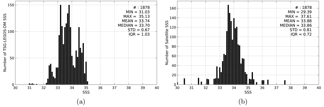
Figure 2: Histograms of SSS from TSG-LEGOS-DM (a) and SMAP-L3-RSS-V2-8DAY-RUNNING-40KM (b) considering all match-up pairs per bins of 0.1 over the Ganga and Brahmaputra river plumes Pi-MEP region and for the full satellite product period.
