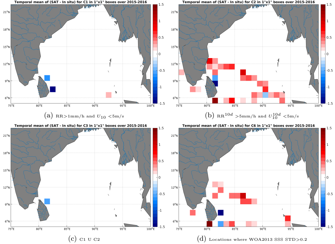
Figure 12: Temporal mean gridded over spatial boxes of size 1^\circ \times 1^\circ of \Delta SSS (SMAP-L3-RSS-V2-8DAY-RUNNING-40KM - TSG-LEGOS-DM) for 4 different subdatasets corresponding to: RR > 1 mm/h and U_{10} < 5 m/s (a), RR^{10d} > 5 mm/h and U_{10}^{10d} < 5 m/s (b), C1 U C2 (c), Locations where WOA2013 SSS STD > 0.2 (d).
