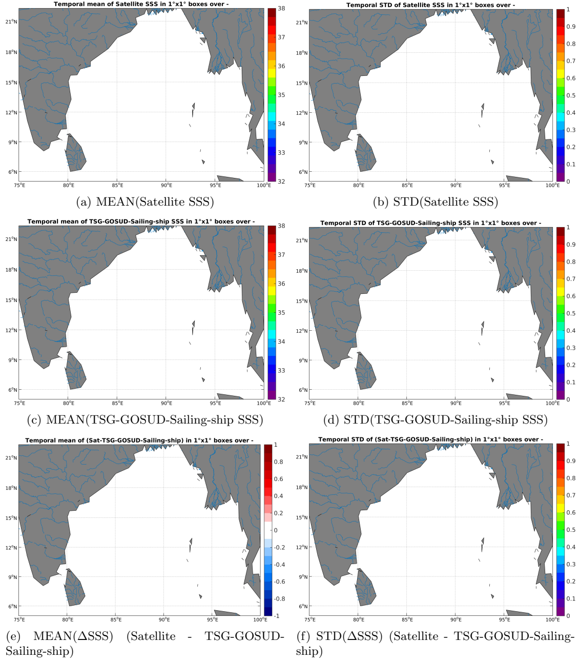
Figure 6: Temporal mean (left) and STD (right) of SSS from SMAP-L3-RSS-V2-8DAY-RUNNING-40KM (top), TSG-GOSUD-Sailing-ship (middle), and of \Delta SSS (Satellite - TSG-GOSUD-Sailing-ship). Only match-up pairs are used to generate these maps.
