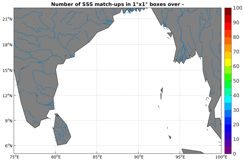
Figure 4: Number of SSS match-ups between TSG-GOSUD-Research-vessel SSS and the SMAP-L3-RSS-V2-8DAY-RUNNING-40KM SSS product for the Ganga and Brahmaputra river plumes Pi-MEP region over 1°x1° boxes and for the full satellite product period.
