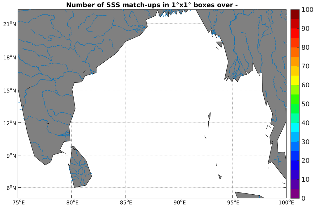
Figure 4: Number of SSS match-ups between Sea mammals SSS and the SMAP-L3-RSS-V2-8DAY-RUNNING-40KM SSS product for the Ganga and Brahmaputra river plumes Pi-MEP region over 1^\circ \times 1^\circ boxes and for the full satellite product period.
