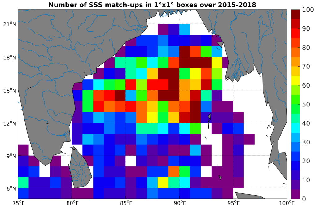
Figure 4: Number of SSS match-ups between Argo SSS and the SMAP-L3-RSS-V2-8DAY-RUNNING-40KM SSS product for the Ganga and Brahmaputra river plumes Pi-MEP region over 1^\circ \times 1^\circ boxes and for the full satellite product period.
