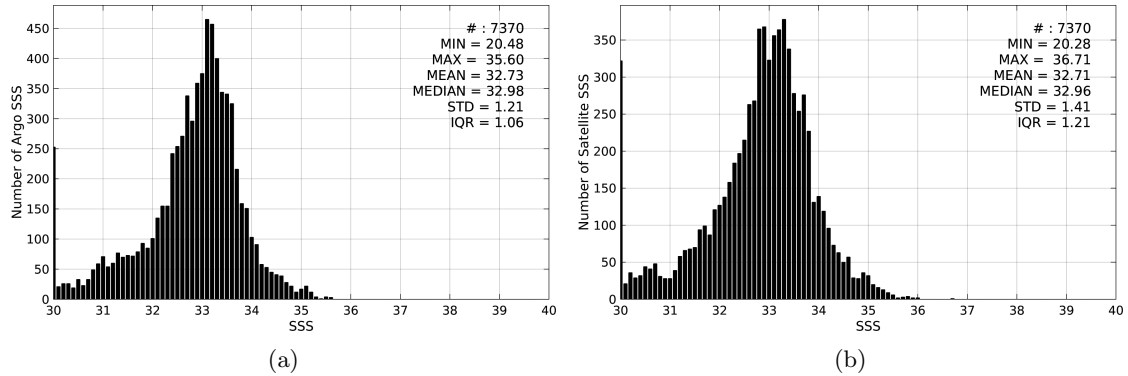
Figure 2: Histograms of SSS from Argo (a) and SMAP-L3-RSS-V2-8DAY-RUNNING-40KM (b) considering all match-up pairs per bins of 0.1 over the Ganga and Brahmaputra river plumes Pi-MEP region and for the full satellite product period.
