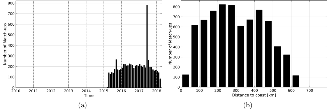
Figure 1: Number of match-ups between Argo and SMAP-L3-RSS-V2-8DAY-RUNNING-40KM SSS as a function of time (a) and as function of the distance to coast (b) over the Ganga and Brahmaputra river plumes Pi-MEP region and for the full satellite product period.
