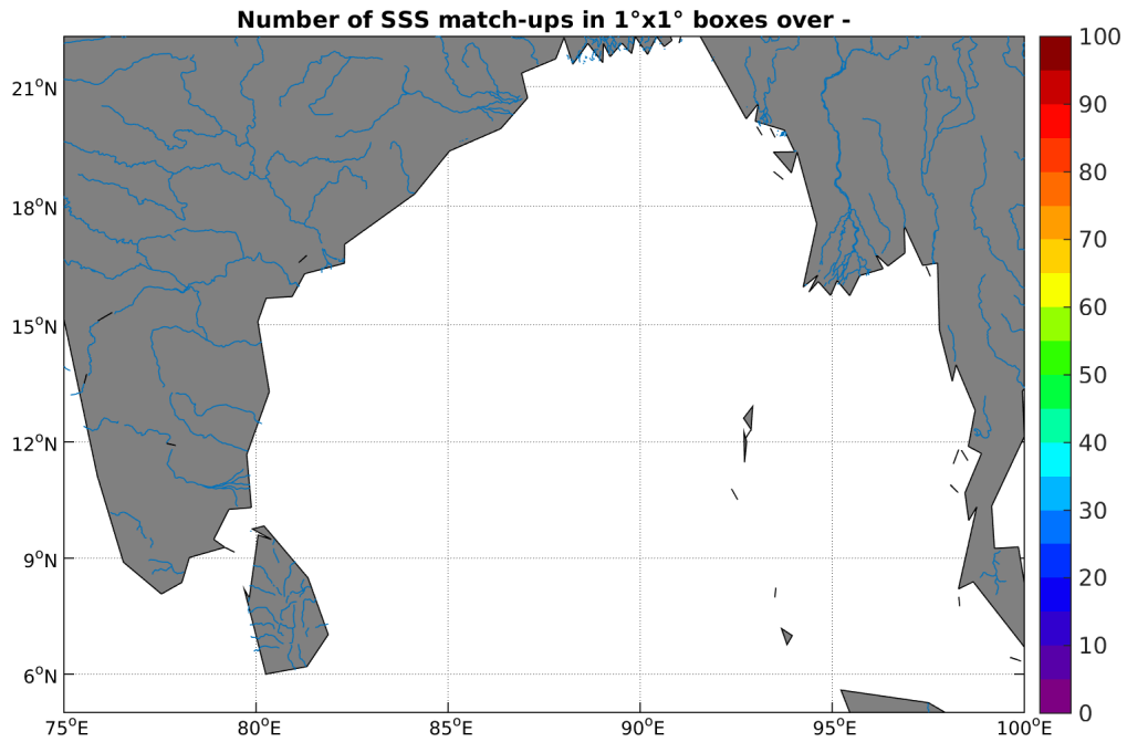
Figure 4: Number of SSS match-ups between TSG-GOSUD-Research-vessel SSS and the SMAP-L3-RSS-V2-8DAY-RUNNING-70KM SSS product for the Ganga and Brahmaputra river plumes Pi-MEP region over 1°x1° boxes and for the full satellite product period.
