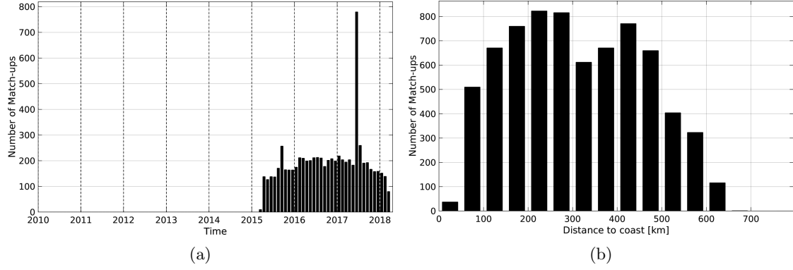
Figure 1: Number of match-ups between Argo and SMAP-L3-RSS-V2-8DAY-RUNNING-70KM SSS as a function of time (a) and as function of the distance to coast (b) over the Ganga and Brahmaputra river plumes Pi-MEP region and for the full satellite product period.
