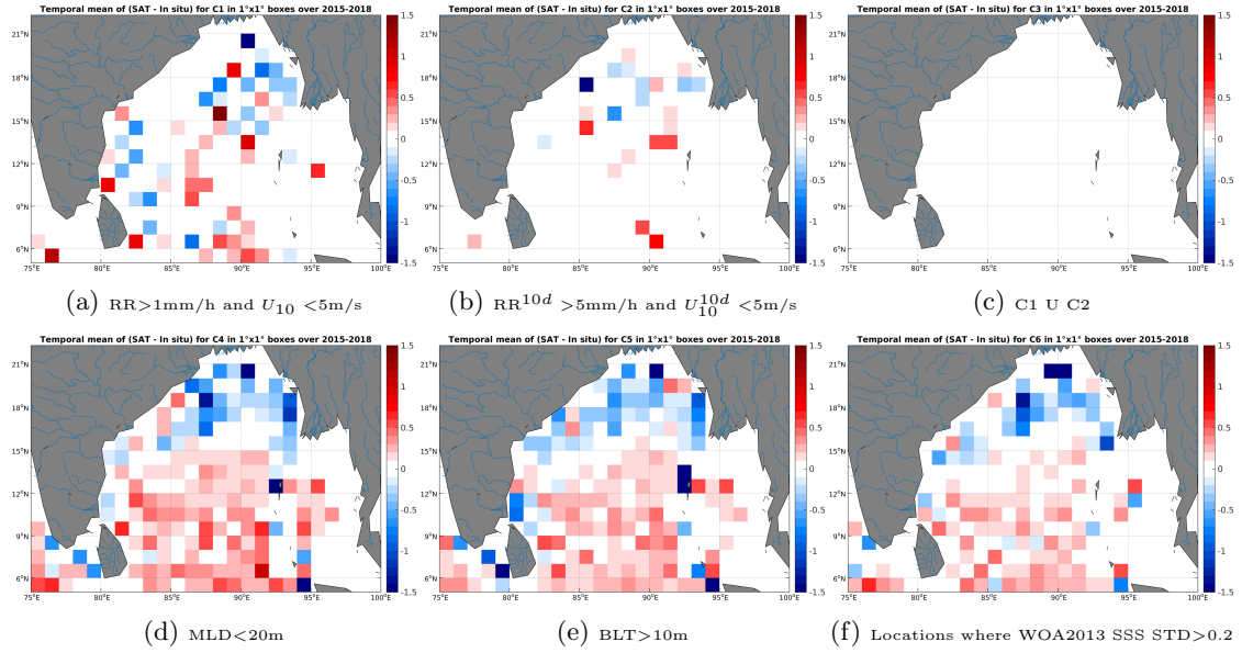
Figure 12: Temporal mean gridded over spatial boxes of size 1^\circ \times 1^\circ of \Delta SSS (SMAP-L3-RSS-V2-8DAY-RUNNING-70KM - Argo) for 6 different subdatasets corresponding to: RR > 1 mm/h and U_{10} < 5 m/s (a), RR^{10d} > 5 mm/h and U_{10}^{10d} < 5 m/s (b), C1 U C2 (c), MLD < 20 m (d), BLT > 10 m (e), Locations where WOA2013 SSS STD > 0.2 (f).
