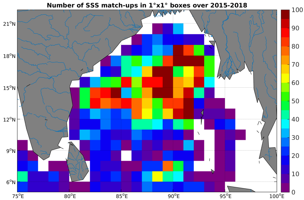
Figure 4: Number of SSS match-ups between Argo SSS and the SMAP-L3-RSS-V2-8DAY-RUNNING-70KM SSS product for the Ganga and Brahmaputra river plumes Pi-MEP region over 1^\circ \times 1^\circ boxes and for the full satellite product period.
