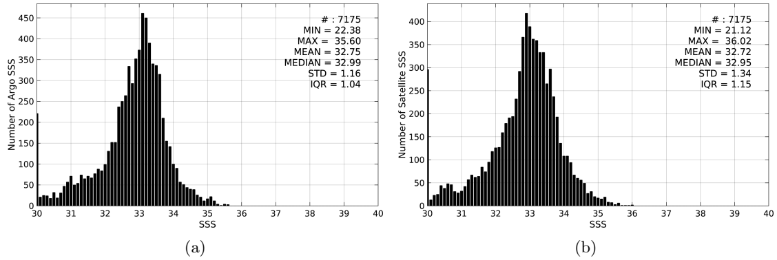
Figure 2: Histograms of SSS from Argo (a) and SMAP-L3-RSS-V2-8DAY-RUNNING-70KM (b) considering all match-up pairs per bins of 0.1 over the Ganga and Brahmaputra river plumes Pi-MEP region and for the full satellite product period.
