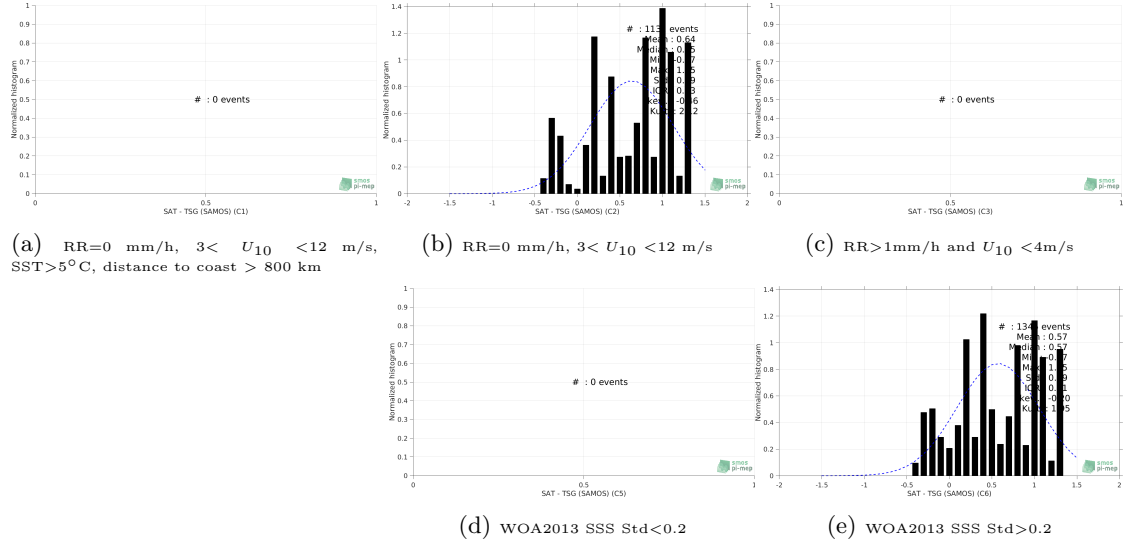
Figure 13: Normalized histogram of \Delta SSS (SMAP SSS L3 v5.0 - 8-Day running (JPL) - TSG (SAMOS)) for 5 different subdatasets corresponding to: RR=0 mm/h, 3 < U_{10} < 12 m/s, SST >5^{\circ} C, distance to coast > 800 km (a), RR=0 mm/h, 3 < U_{10} < 12 m/s (b), RR >1 mm/h and U_{10} < 4 m/s (c), WOA2013 SSS Std <0.2 (d), WOA2013 SSS Std >0.2 (e).
