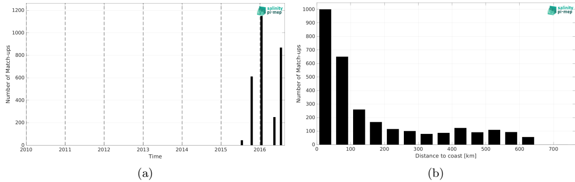
Figure 2: Number of match-ups between TSG (LEGOS-DM) and SMAP SSS L3 v5.0 - 8-Day running (JPL) SSS as a function of time (a) and as function of the distance to coast (b) over the Ganga and Brahmaputra river plumes Pi-MEP region and for the full satellite product period.
