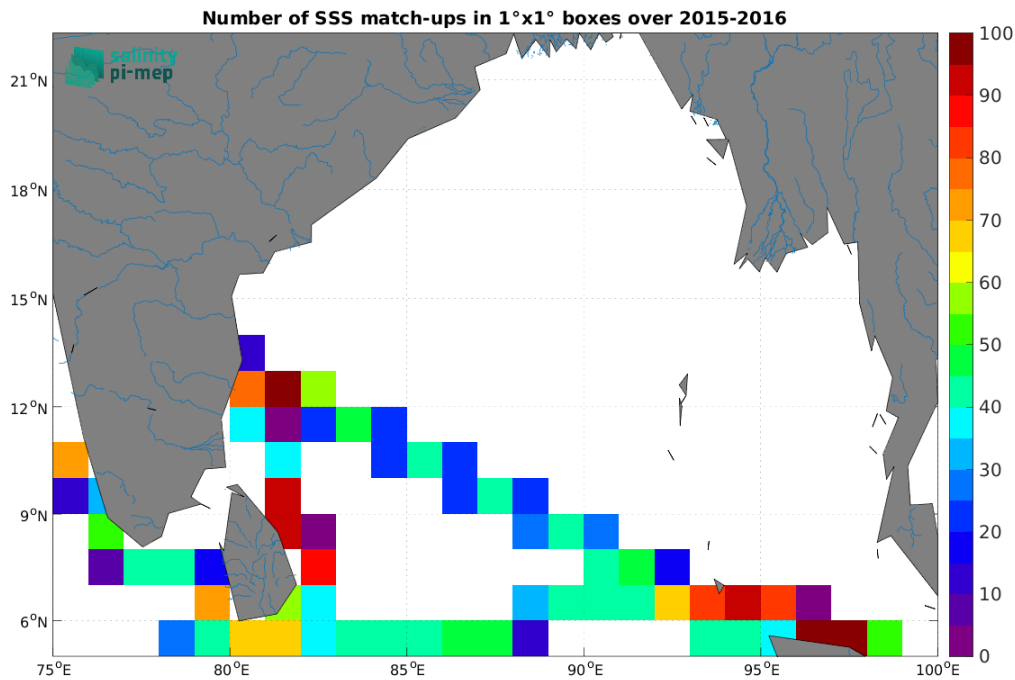
Figure 5: Number of SSS match-ups between TSG (LEGOS-DM) SSS and the SMAP SSS L3 v5.0 - 8-Day running (JPL) SSS product for the Ganga and Brahmaputra river plumes Pi-MEP region over 1^\circ \times 1^\circ boxes and for the full satellite product period.
