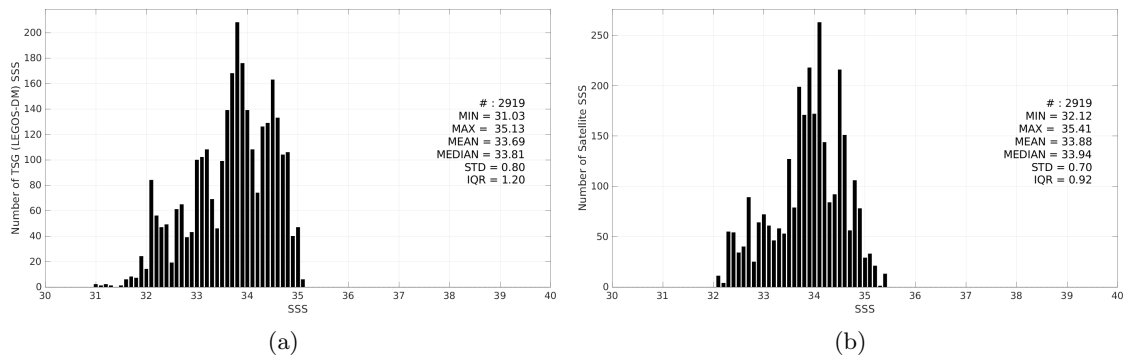
Figure 3: Histograms of SSS from TSG (LEGOS-DM) (a) and SMAP SSS L3 v5.0 - 8-Day running (JPL) (b) considering all match-up pairs per bins of 0.1 over the Ganga and Brahmaputra river plumes Pi-MEP region and for the full satellite product period.
