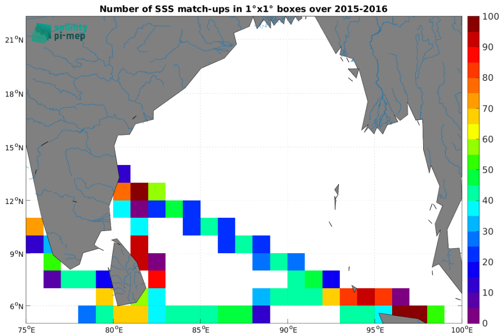
Figure 4: Number of SSS match-ups between TSG (LEGOS-DM) SSS and the SMAP SSS L3 v5.0 - 8-Day running (JPL) SSS product for the Ganga and Brahmaputra river plumes Pi-MEP region over 1^\circ \times 1^\circ boxes and for the full satellite product period.
