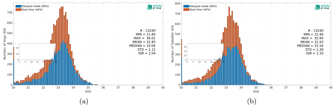
Figure 3: Histograms of SSS from Argo (a) and SMAP SSS L3 v5.0 - 8-Day running (JPL) (b) considering all match-up pairs per bins of 0.1 over the Ganga and Brahmaputra river plumes Pi-MEP region and for the full satellite product period.
