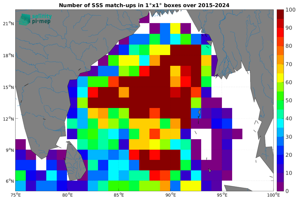
Figure 5: Number of SSS match-ups between Argo SSS and the SMAP SSS L3 v5.0 - 8-Day running (JPL) SSS product for the Ganga and Brahmaputra river plumes Pi-MEP region over 1^\circ \times 1^\circ boxes and for the full satellite product period.
