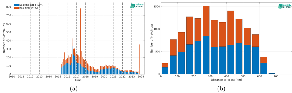
Figure 2: Number of match-ups between Argo and SMAP SSS L3 v5.0 - 8-Day running (JPL) SSS as a function of time (a) and as function of the distance to coast (b) over the Ganga and Brahmaputra river plumes Pi-MEP region and for the full satellite product period.
