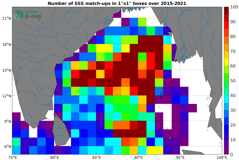
Figure 4: Number of SSS match-ups between Argo SSS and the SMAP SSS L3 v5.0 - 8-Day running (JPL) SSS product for the Ganga and Brahmaputra river plumes Pi-MEP region over 1^{\circ} \times 1^{\circ} boxes and for the full satellite product period.
