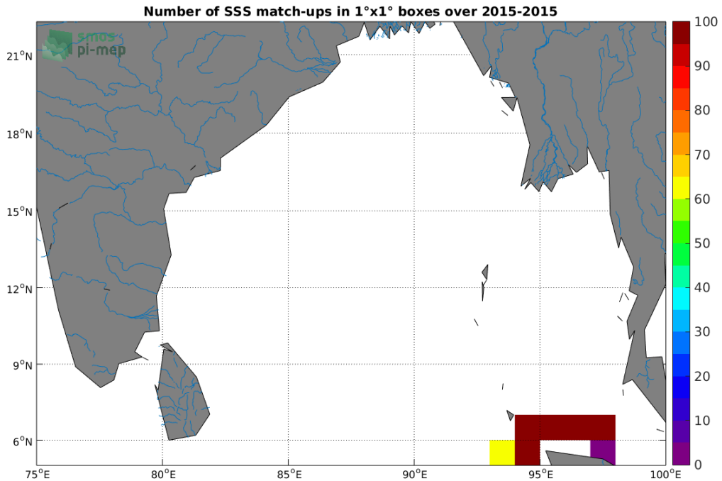
Figure 4: Number of SSS match-ups between TSG-SAMOS SSS and the SMAP-L3-JPL-V4.3-8DAY-RUNNING-60KM SSS product for the Ganga and Brahmaputra river plumes Pi-MEP region over 1°x1° boxes and for the full satellite product period.
