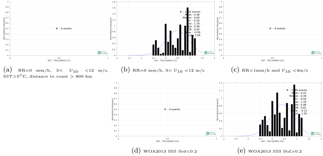
Figure 13: Normalized histogram of \Delta SSS (SMAP-L3-JPL-V4.3-8DAY-RUNNING-60KM - TSG-SAMOS) for 5 different subdatasets corresponding to: RR=0 mm/h, 3 < U_{10} < 12 m/s, SST>5°C, distance to coast > 800 km (a), RR=0 mm/h, 3 < U_{10} < 12 m/s (b), RR>1mm/h and U_{10} < 4 m/s (c), WOA2013 SSS Std<0.2 (d), WOA2013 SSS Std>0.2 (e).
