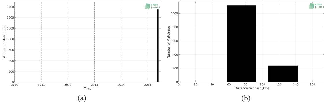
Figure 1: Number of match-ups between TSG-SAMOS and SMAP-L3-JPL-V4.3-8DAY-RUNNING-60KM SSS as a function of time (a) and as function of the distance to coast (b) over the Ganga and Brahmaputra river plumes Pi-MEP region and for the full satellite product period.
