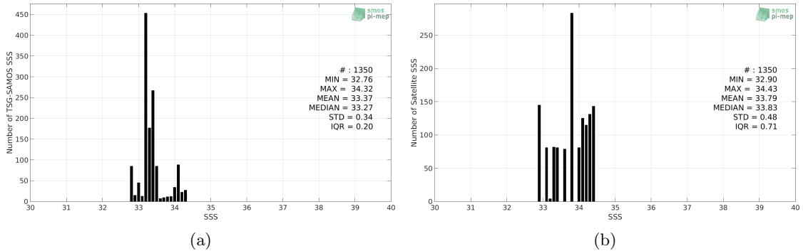
Figure 2: Histograms of SSS from TSG-SAMOS (a) and SMAP-L3-JPL-V4.3-8DAY-RUNNING-60KM (b) considering all match-up pairs per bins of 0.1 over the Ganga and Brahmaputra river plumes Pi-MEP region and for the full satellite product period.
