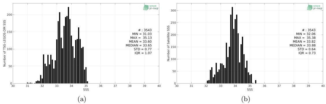
Figure 2: Histograms of SSS from TSG-LEGOS-DM (a) and SMAP-L3-JPL-V4.3-8DAY-RUNNING-60KM (b) considering all match-up pairs per bins of 0.1 over the Ganga and Brahmaputra river plumes Pi-MEP region and for the full satellite product period.
