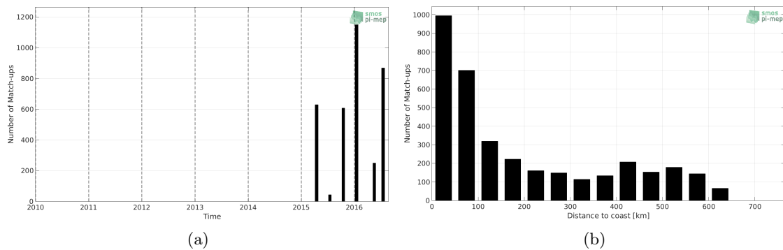
Figure 1: Number of match-ups between TSG-LEGOS-DM and SMAP-L3-JPL-V4.3-8DAY-RUNNING-60KM SSS as a function of time (a) and as function of the distance to coast (b) over the Ganga and Brahmaputra river plumes Pi-MEP region and for the full satellite product period.
