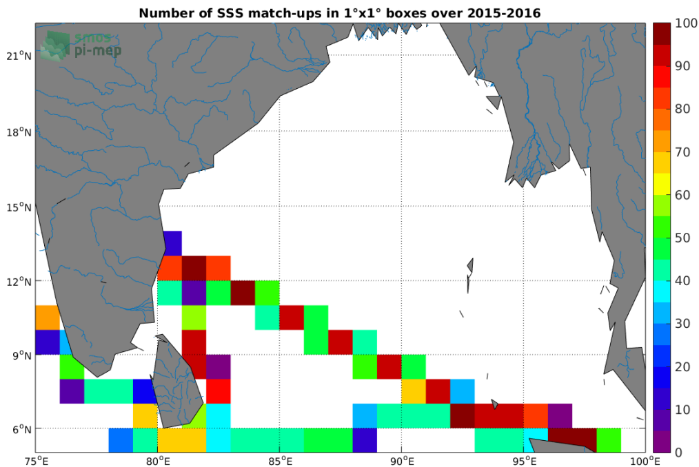
Figure 4: Number of SSS match-ups between TSG-LEGOS-DM SSS and the SMAP-L3-JPL-V4.3-8DAY-RUNNING-60KM SSS product for the Ganga and Brahmaputra river plumes Pi-MEP region over 1°x1° boxes and for the full satellite product period.
