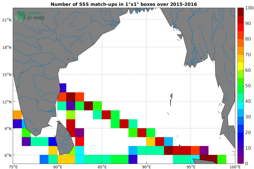
Figure 4: Number of SSS match-ups between TSG-LEGOS-DM SSS and the SMAP-L3-JPL-V4.3-8DAY-RUNNING-60KM SSS product for the Ganga and Brahmaputra river plumes Pi-MEP region over 1^\circ \times 1^\circ boxes and for the full satellite product period.
