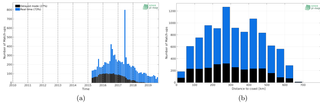
Figure 1: Number of match-ups between Argo and SMAP-L3-JPL-V4.3-8DAY-RUNNING-60KM SSS as a function of time (a) and as function of the distance to coast (b) over the Ganga and Brahmaputra river plumes Pi-MEP region and for the full satellite product period.
