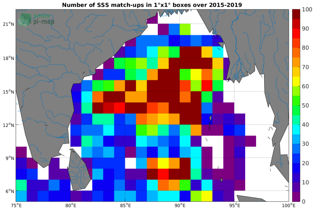
Figure 4: Number of SSS match-ups between Argo SSS and the SMAP-L3-JPL-V4.3-8DAY-RUNNING-60KM SSS product for the Ganga and Brahmaputra river plumes Pi-MEP region over 1°x1° boxes and for the full satellite product period.
