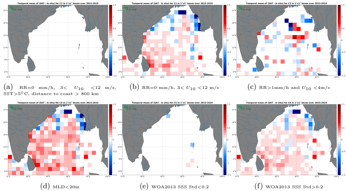
Figure 12: Temporal mean gridded over spatial boxes of size 1^\circ \times 1^\circ of \Delta SSS (SMAP-L3-JPL-V4.3-8DAY-RUNNING-60KM - Argo) for 6 different subdatasets corresponding to:RR=0 mm/h, 3 < U_{10} < 12 m/s, SST >5^\circ C, distance to coast > 800 km (a), RR=0 mm/h, 3 < U_{10} < 12 m/s (b), RR >1 mm/h and U_{10} < 4 m/s (c),MLD <20 m (d),WOA2013 SSS Std <0.2 (e),WOA2013 SSS Std >0.2 (f).
