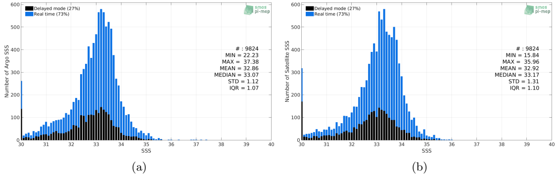
Figure 2: Histograms of SSS from Argo (a) and SMAP-L3-JPL-V4.3-8DAY-RUNNING-60KM (b) considering all match-up pairs per bins of 0.1 over the Ganga and Brahmaputra river plumes Pi-MEP region and for the full satellite product period.
