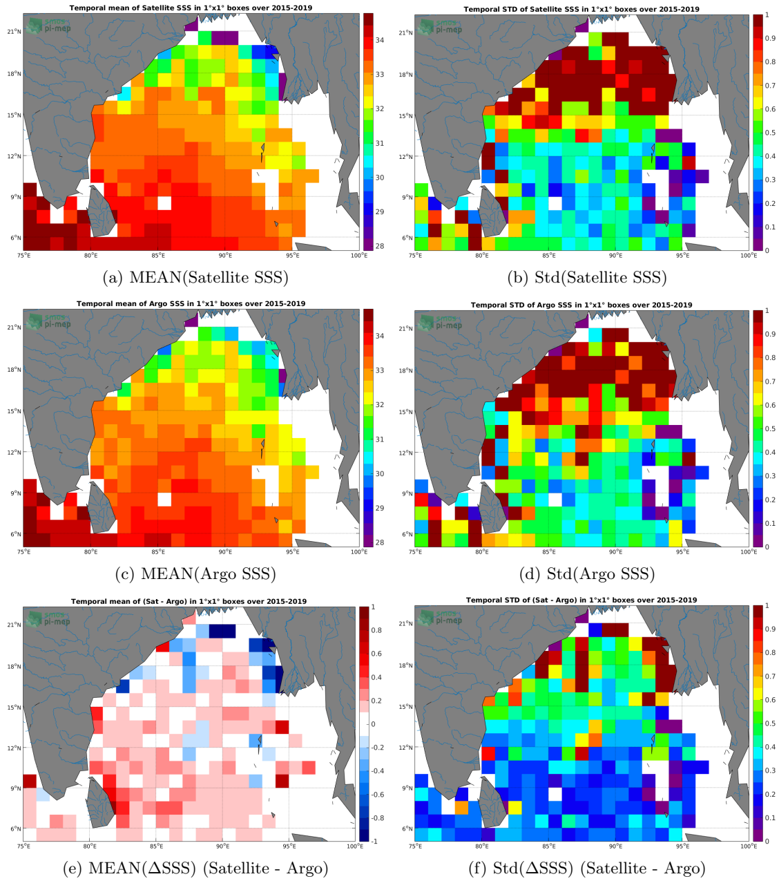
Figure 6: Temporal mean (left) and Std (right) of SSS from SMAP-L3-JPL-V4.3-8DAY-RUNNING-60KM (top), Argo (middle), and of \Delta SSS (Satellite - Argo). Only match-up pairs are used to generate these maps.
