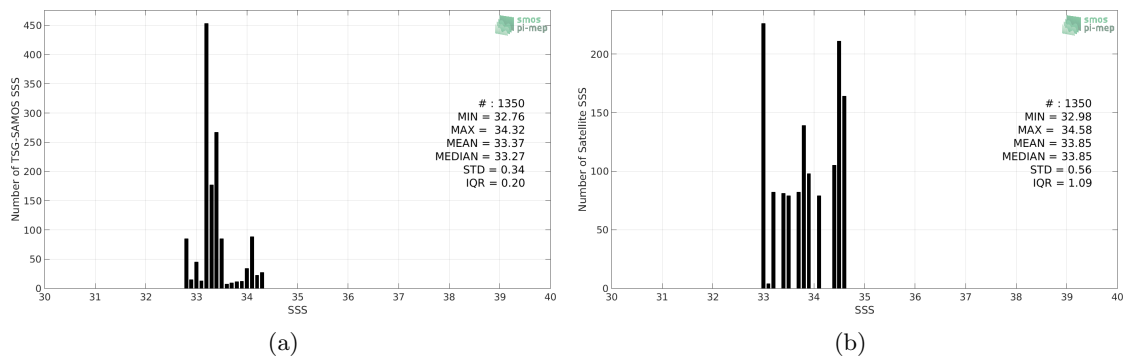
Figure 2: Histograms of SSS from TSG-SAMOS (a) and SMAP-L3-JPL-V4.3-MONTHLY-60KM (b) considering all match-up pairs per bins of 0.1 over the Ganga and Brahmaputra river plumes Pi-MEP region and for the full satellite product period.
