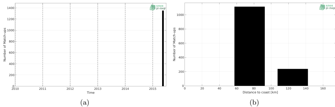
Figure 1: Number of match-ups between TSG-SAMOS and SMAP-L3-JPL-V4.3-MONTHLY-60KM SSS as a function of time (a) and as function of the distance to coast (b) over the Ganga and Brahmaputra river plumes Pi-MEP region and for the full satellite product period.
