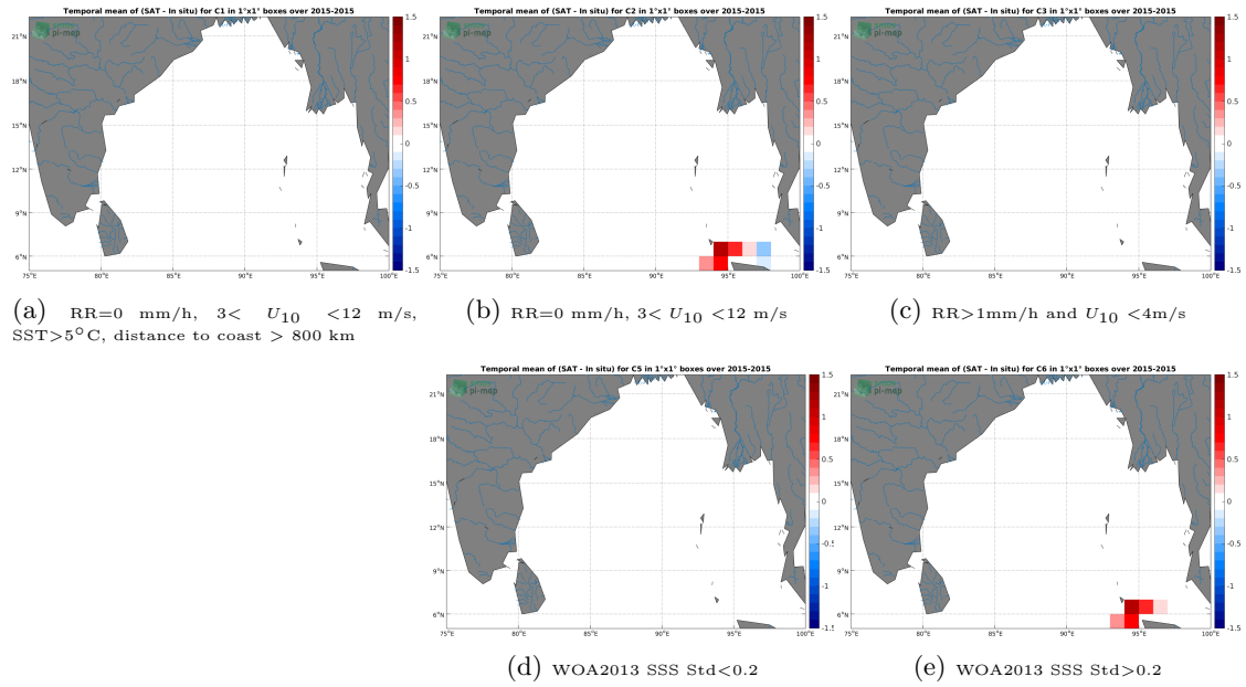
Figure 12: Temporal mean gridded over spatial boxes of size 1^\circ \times 1^\circ of \Delta SSS (SMAP-L3-JPL-V4.3-MONTHLY-60KM - TSG-SAMOS) for 5 different subdatasets corresponding to:RR=0 mm/h, 3 < U_{10} < 12 m/s, SST >5^\circ C, distance to coast > 800 km (a), RR=0 mm/h, 3 < U_{10} < 12 m/s (b), RR >1 mm/h and U_{10} < 4 m/s (c), WOA2013 SSS Std <0.2 (d), WOA2013 SSS Std >0.2 (e).
