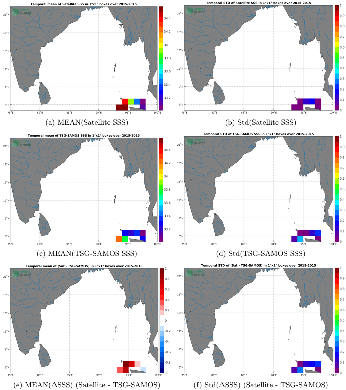
Figure 6: Temporal mean (left) and Std (right) of SSS from SMAP-L3-JPL-V4.3-MONTHLY-60KM (top), TSG-SAMOS (middle), and of \Delta SSS (Satellite - TSG-SAMOS). Only match-up pairs are used to generate these maps.
